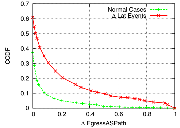
Fig. 9. Egress router and AS path shifts ( \Delta EgressASPath ).
