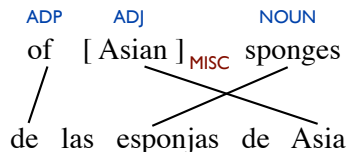
Figure 1: An English (top) – Spanish (bottom) phrase pair from our parallel data. The correct POS tags and NER annotations are shown for the English phrase. Word alignments are shown as links between English and Spanish words.
