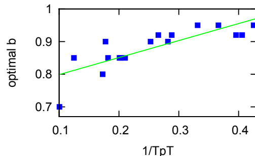
Figure 2: Correlation between optimal constraint value b and dictionary pruning efficiency. Each blue square is a language, the green line is a linear approximation of the data.
