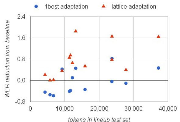
Figure 2: WER reduction vs. number of tokens in the test set, for both one-best and lattice-based adaptation for each of the lineups examined.
