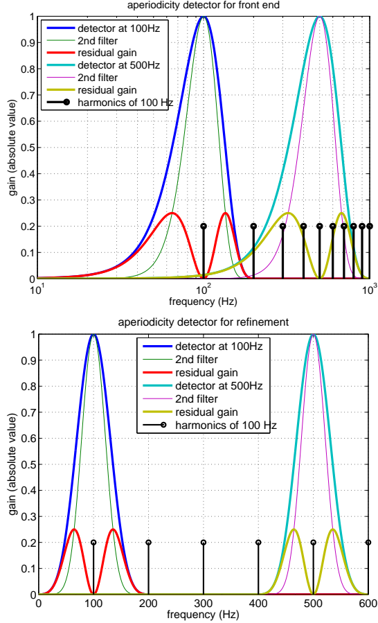
Figure 9: Detector allocation of the front end (upper plot) and the refinement stage (lower plot).
