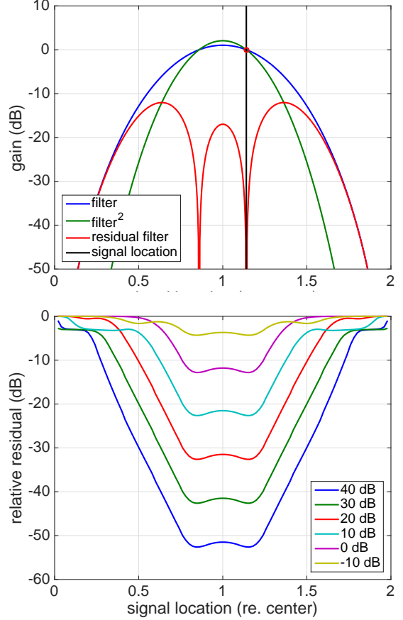
Figure 8: principles of operation. Upper plot shows filter shape and the dominant signal at 1.14f_c . Filter gains are adjusted to make output levels are 0 dB. Subtracting the second filter gain from the first one yields the equivalent filter for other components. Lower plot shows the output residual level as a function of the location of the dominant signal and the noise level.
