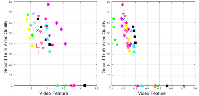
Fig. 1. Along the X-axis of these scatter plots are the (Left) aggregated (GGD) shape features and (Right) self-referenced video quality features. Along the Y-axis are the ground truth quality scores of 50 videos in the LIVE VQA Database [11]
