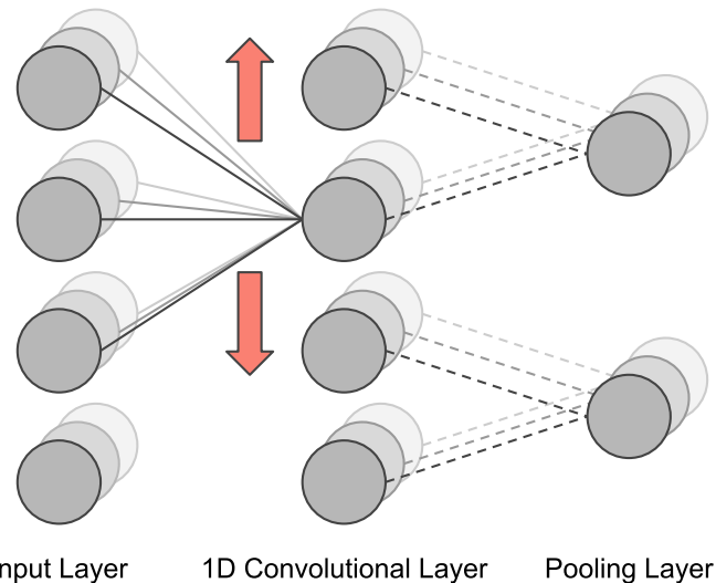
Figure 2. Three layers of a one-dimensional convolutional neural network. The convolutional layer takes the discrete cross-correlation operation of the vectors in its input layer with kernel vectors that are learned by the model. The pooling layer aggregates values in small neighborhoods along its input, typically by taking the mean or maximum value within each neighborhood. The pooling layer aggregates regions spaced s neurons apart, where s is the stride length ; here, the stride length is 2.
