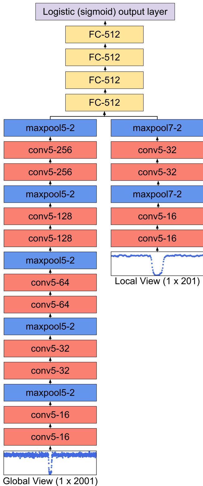
Figure 7. Architecture of our best-performing neural network model. Convolutional layers are denoted conv (kernel size)-(number of feature maps), max pooling layers are denoted maxpool (window length)-(stride length), and fully connected layers are denoted FC-(number of units).
