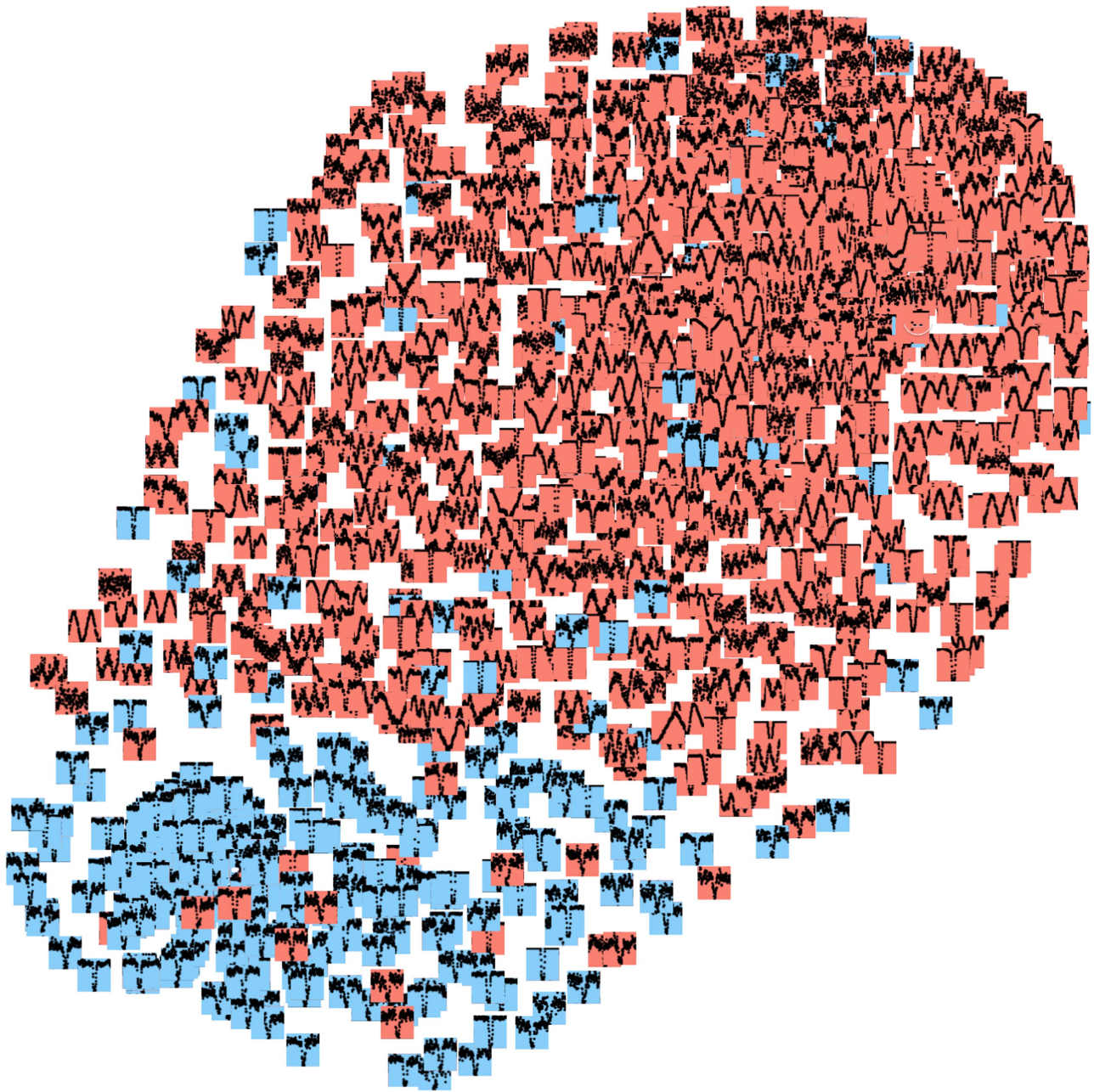
Figure 9. Visualizing the geometric space in which our convolutional neural network embeds its input light curves. We used the t-SNE algorithm for dimensionality reduction to create a two-dimensional embedding such that light curves that are close in the original space are also close in the 2D space. Light curves that are far apart in 2D space are not necessarily far apart in the original space. Notice that true planet candidates (blue) are close to other planet candidates, and false positives (red) are close to similarly shaped false positives.
