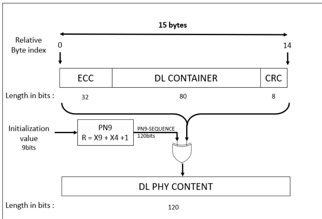
Figure 4-6: Whitening function in DL
