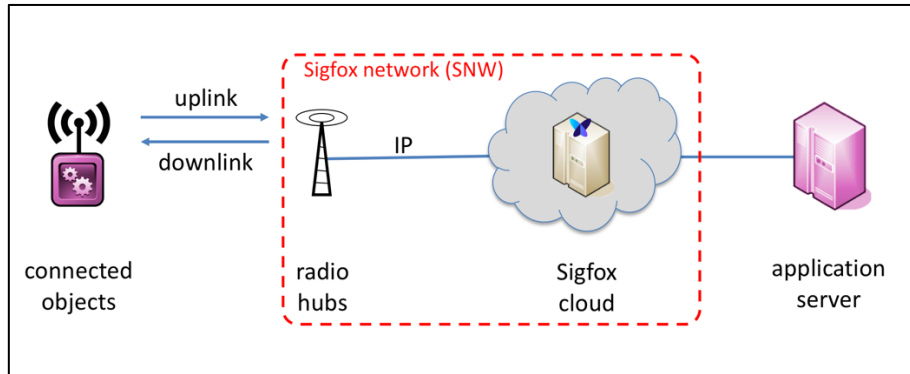
Figure 1-1 : Radio interface
