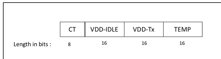
Figure 5-1 : Payload of a keep-alive control message
