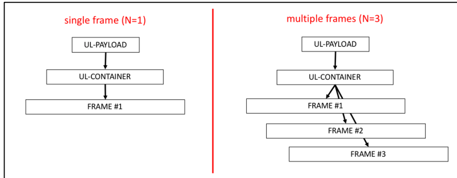
Figure 3-7: Principle of multiple transmissions in uplink
