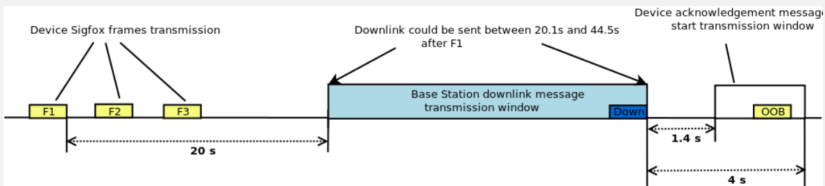
Figure 1: Downlink Timings
