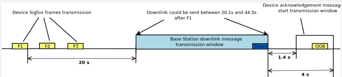
Figure 1: Downlink Timings
