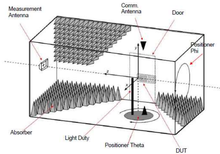
Figure 2: Coordinate system anechoic chamber (OTA)
