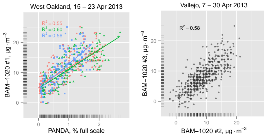
Fig. 3. Left: 1 h data collected between 15–23 April 2013 from three PANDAs and a reference ( \beta -attenuation) \text{PM}_{2.5} instrument at the regulatory monitoring site in Oakland. Right: approximately the same level of agreement ( R^2 \approx 0.6 ) was found between 1 h data from a pair of \beta -attenuation instruments at a nearby regulatory monitoring site in Vallejo, California (40 km away), 7–30 April 2013. The original 1 h BAM data were available only at 1 \mu\text{g m}^{-3} resolution; points are jittered to reduce overplotting. Superimposed lines represent linear regressions of unjittered 1 h data.
