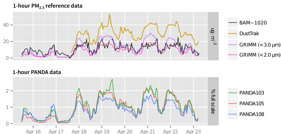
Fig. 1. Hourly data collected between 15 April 2013 and 23 April 2013 at the West Oakland regulatory monitoring site. Top: \text{PM}_{2.5} measurements reported by BAM-1020, DustTrak, and GRIMM. Bottom: output (% full scale) from three Shinyei PPD42NS sensors (see Table S1 and Figs. S1, S2, and S3, Supplement, for configuration details).
