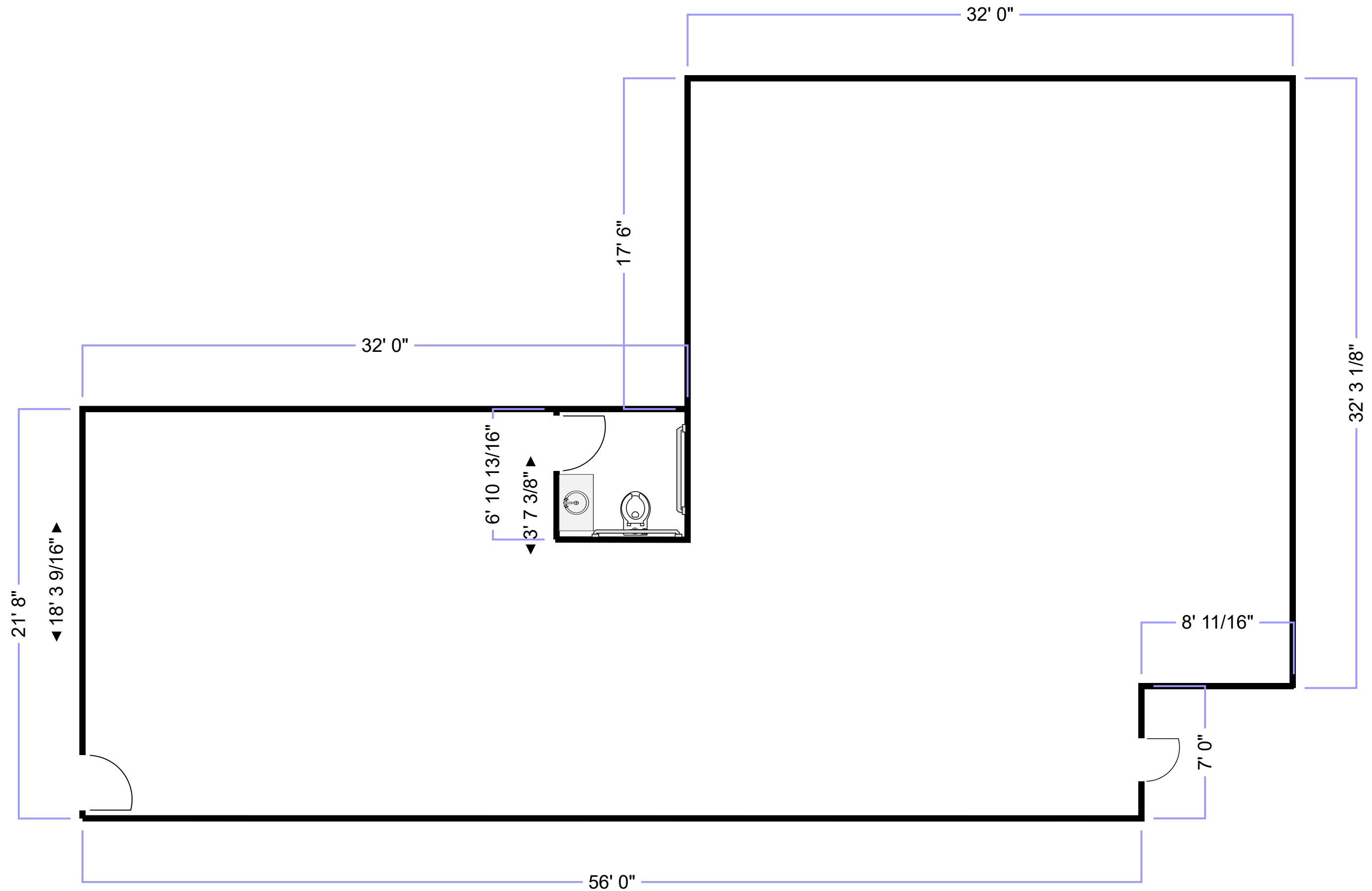
6301 3A - Open Floor Plan (Current)
