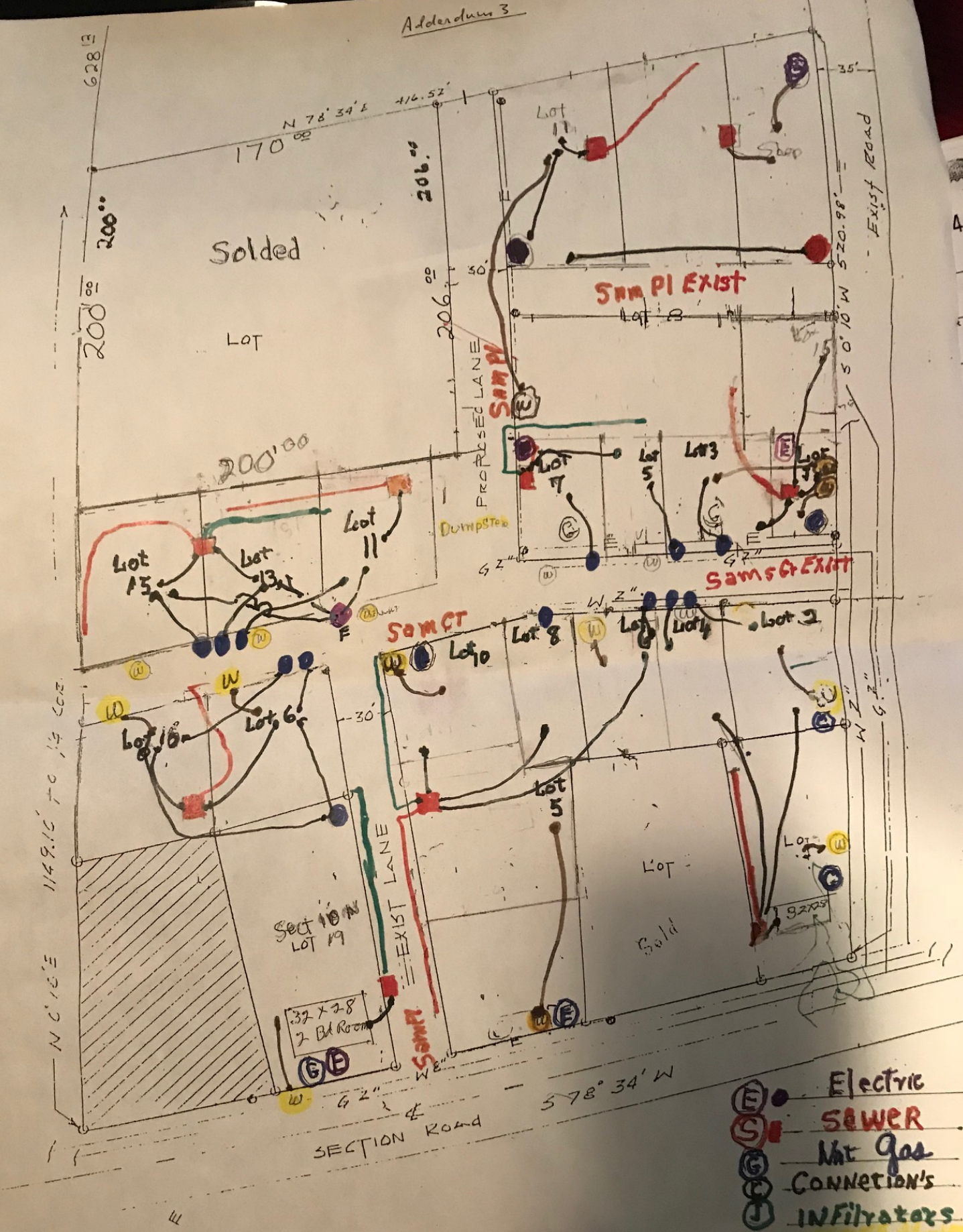
SAM'S PLACE - Proposed Plat SCALE 1982 By Sam 1" = 50'
