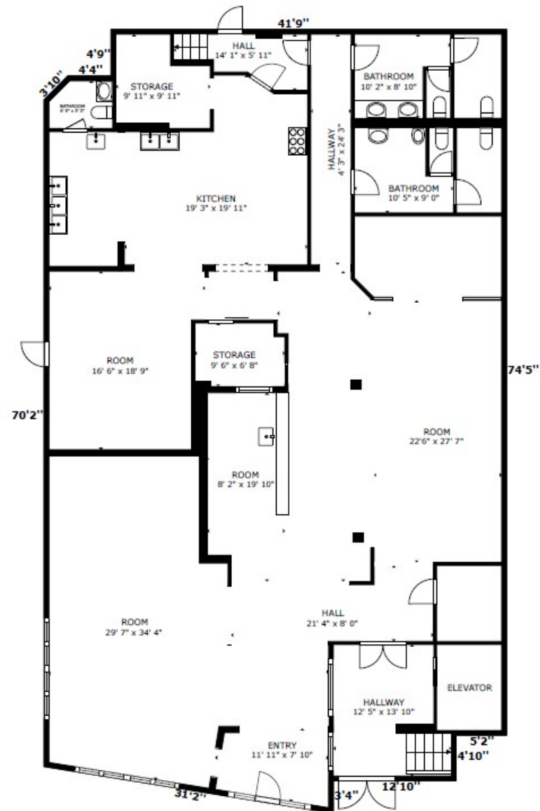
FLOOR 1
