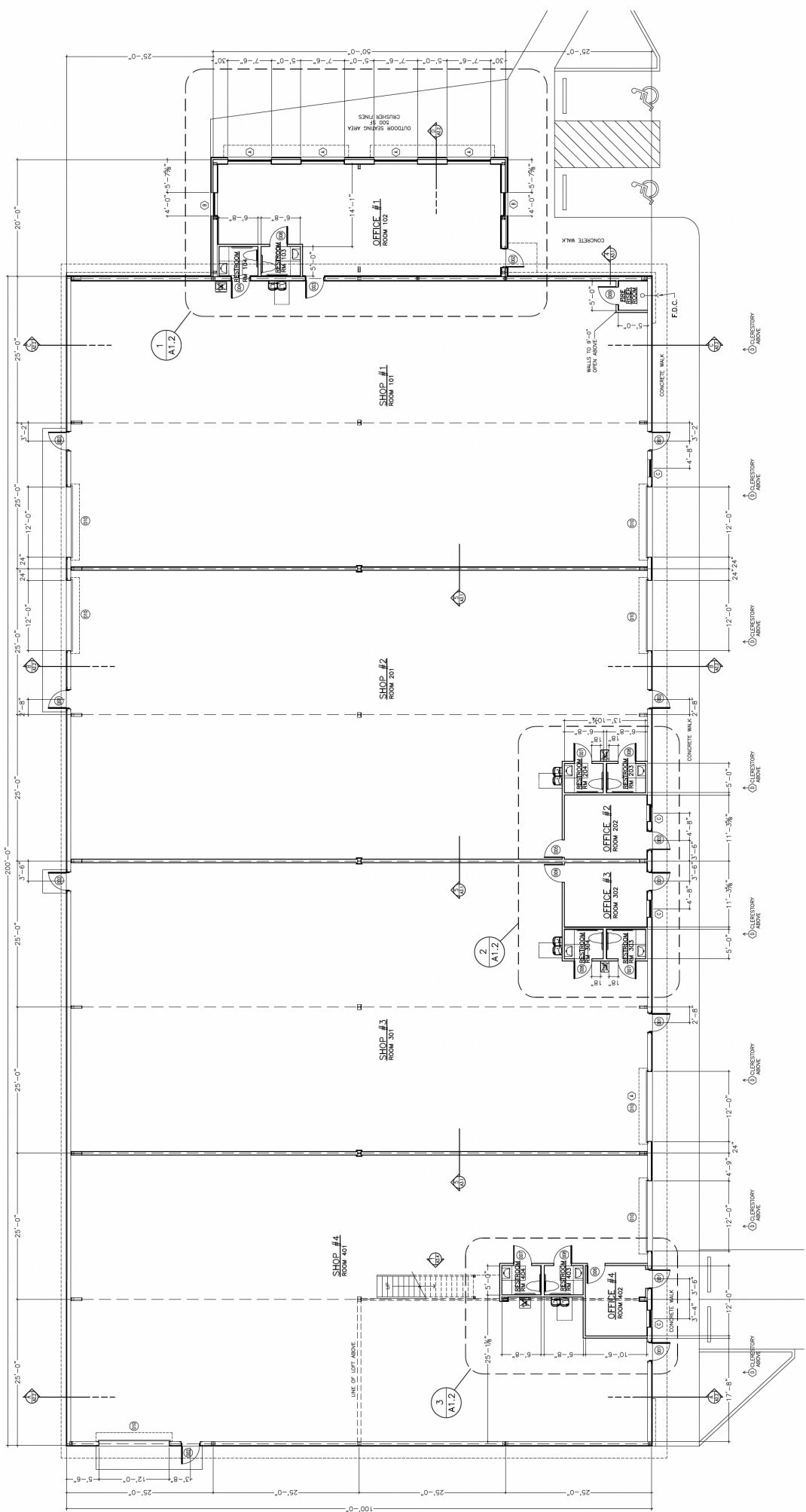
FLOOR PLAN 1/8" = 1'-0"
