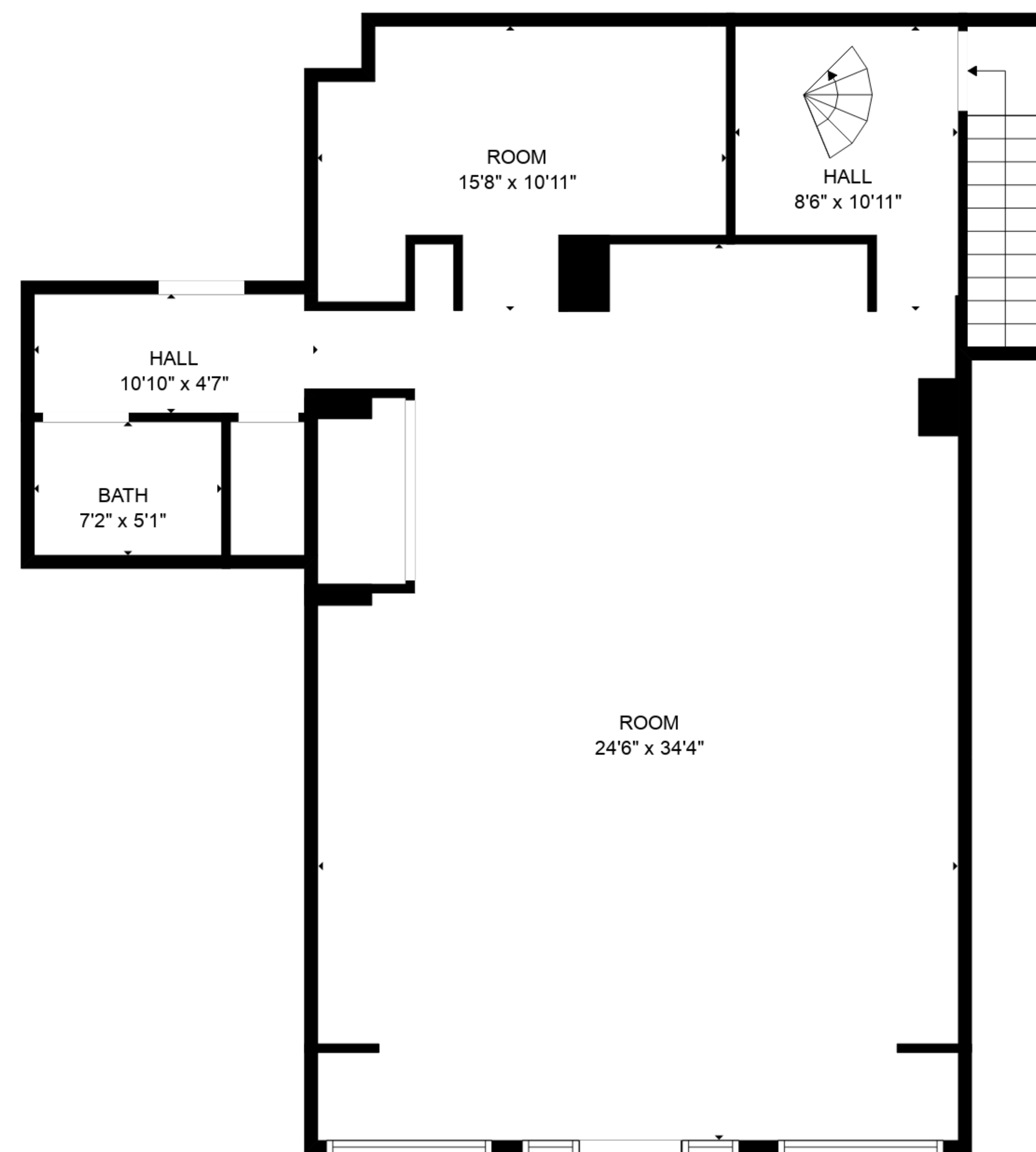
FLOOR 2
