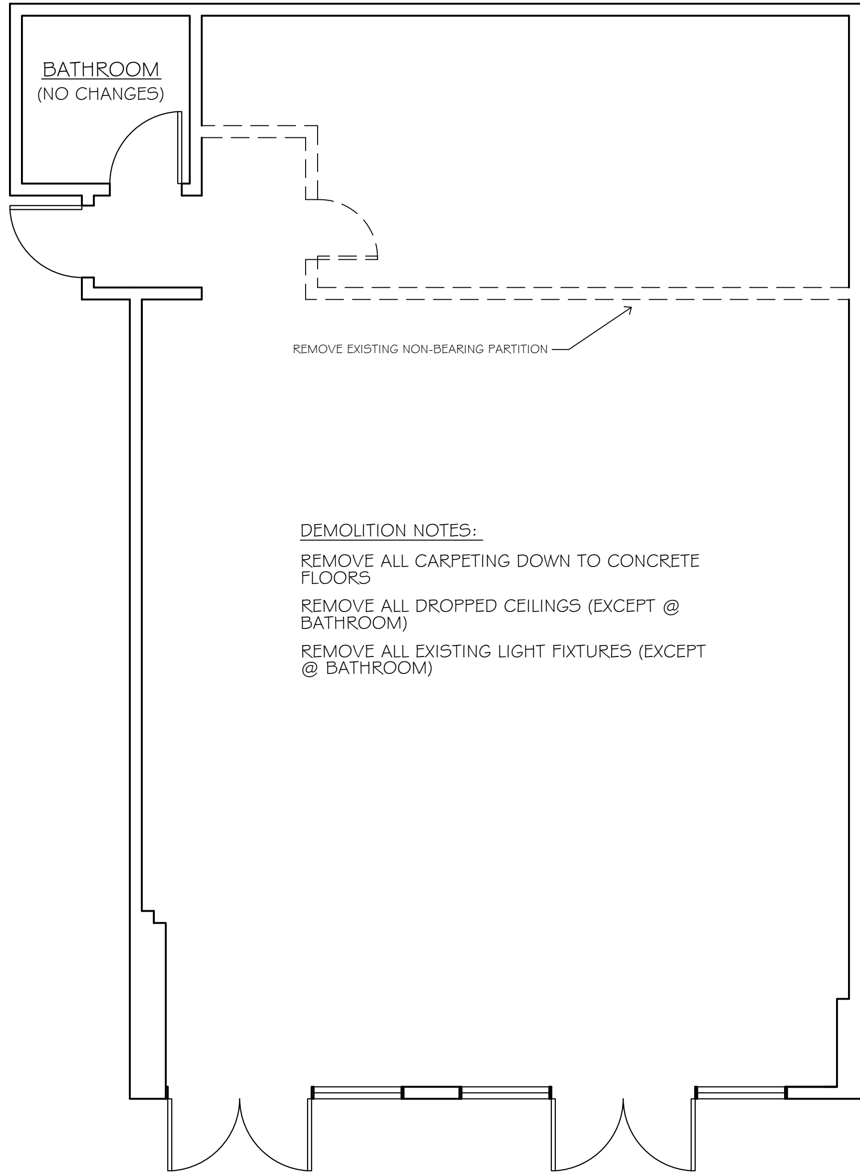
EXISTING FLOOR PLAN SCALE: 1/4" = 1'-0"
