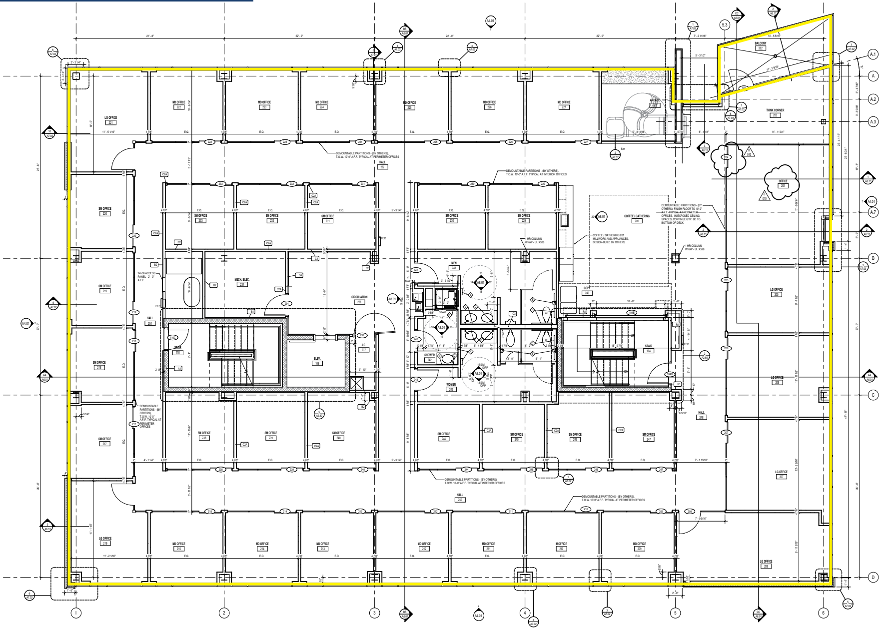
SECOND FLOOR 1/4" = 1'-0"
