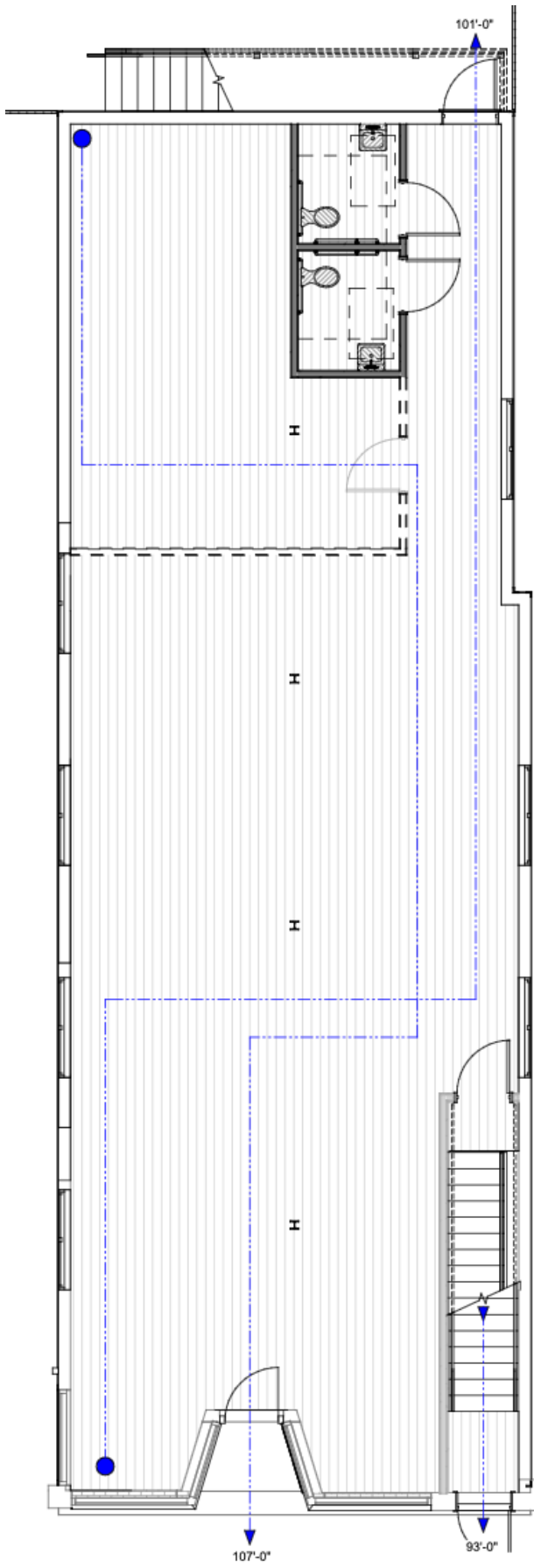
Main Level
