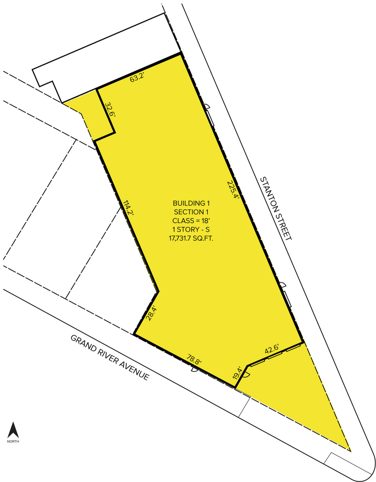
Site Plan
