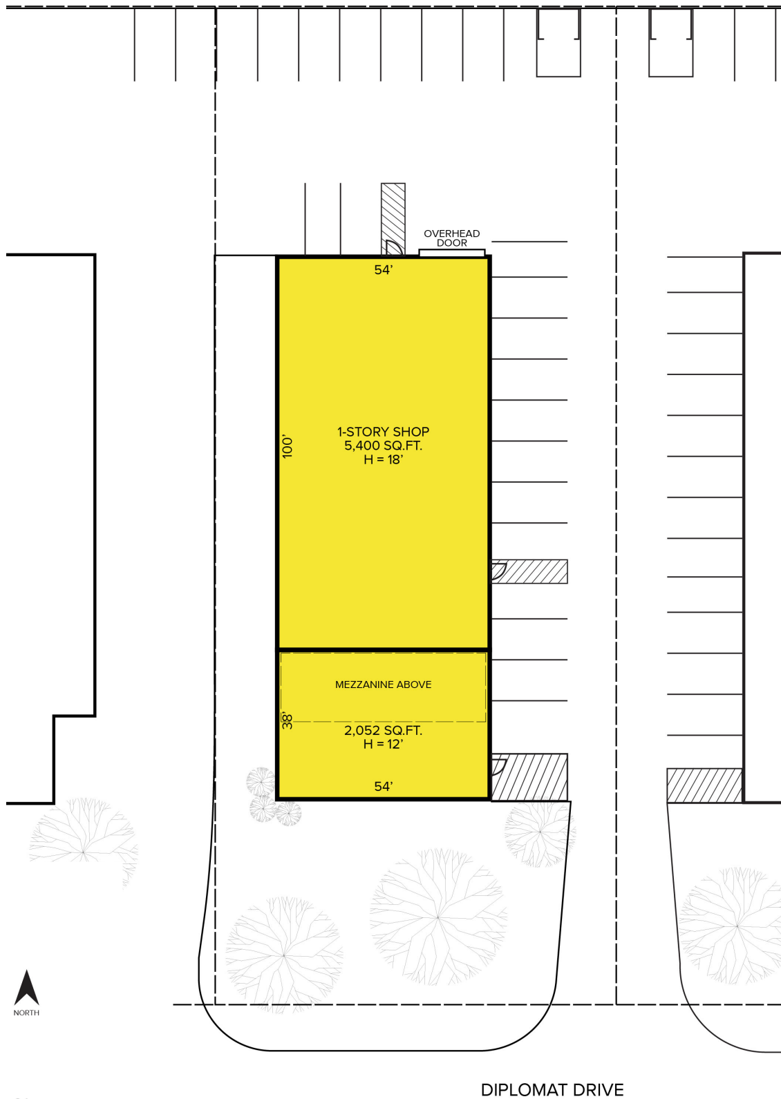
Site Plan
