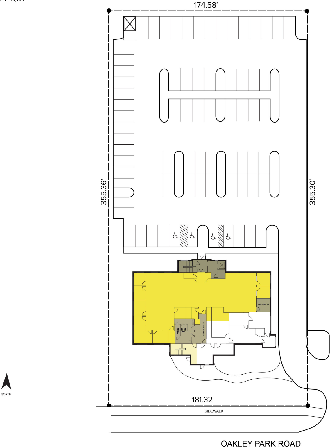
Site Plan
