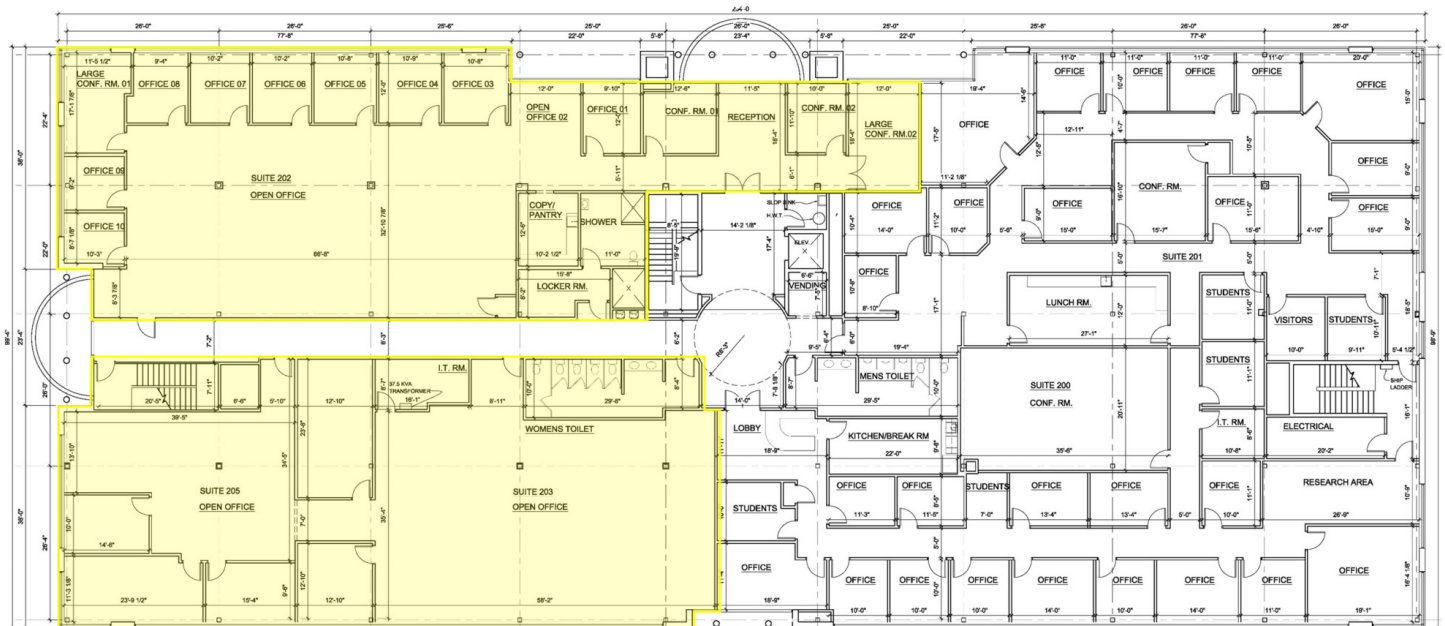
1 A.2 EXISTING SECOND FLOOR PLAN 18' x 110'
