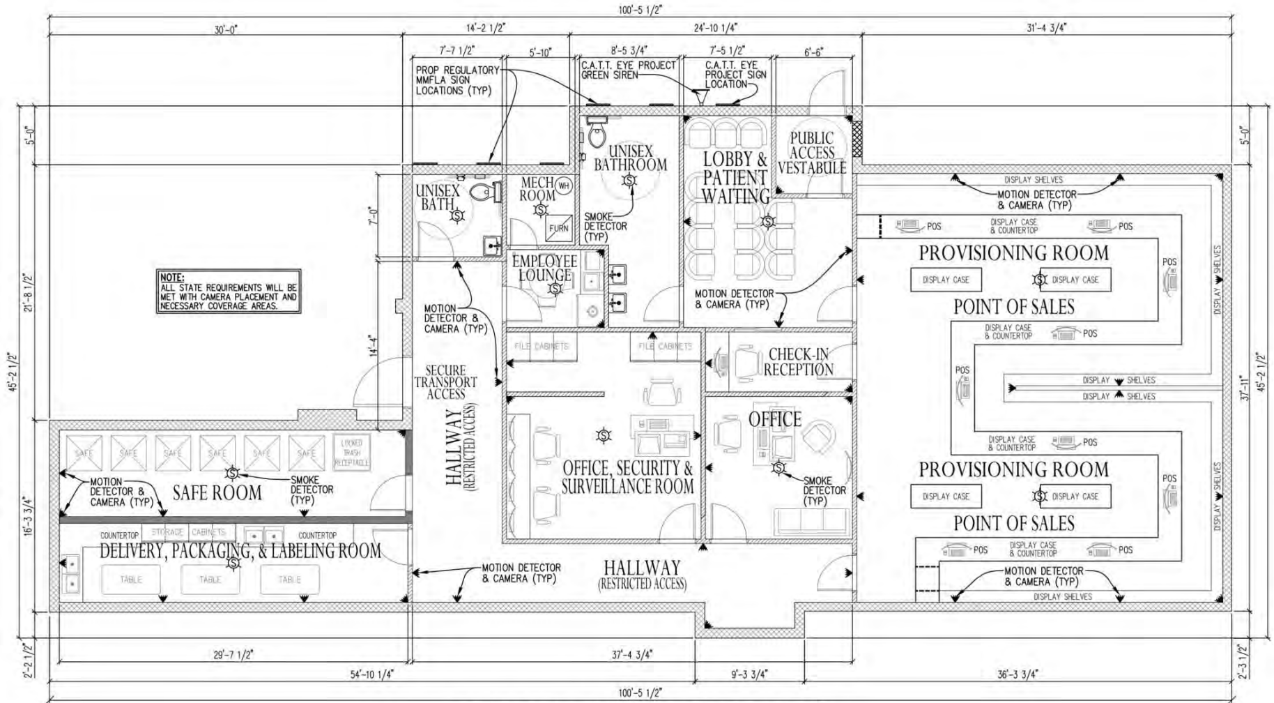
PROPOSED BUILDING FLOOR PLAN
