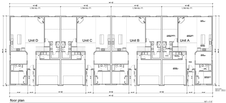
floor plan
