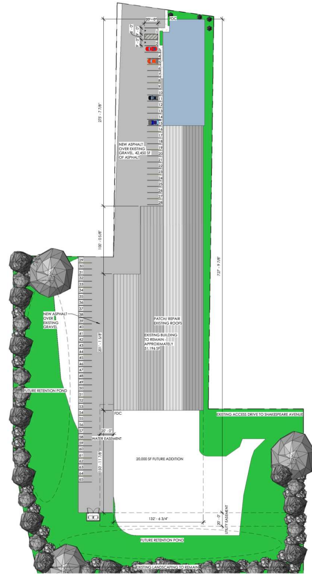
1 PROPOSED SITE PLAN C100 1" = 40'-0"
