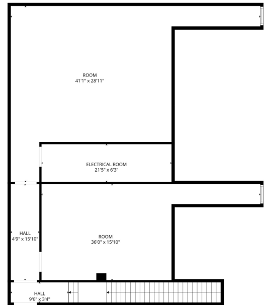
UPSTAIRS ADDITIONAL SQUARE FOOTAGE
