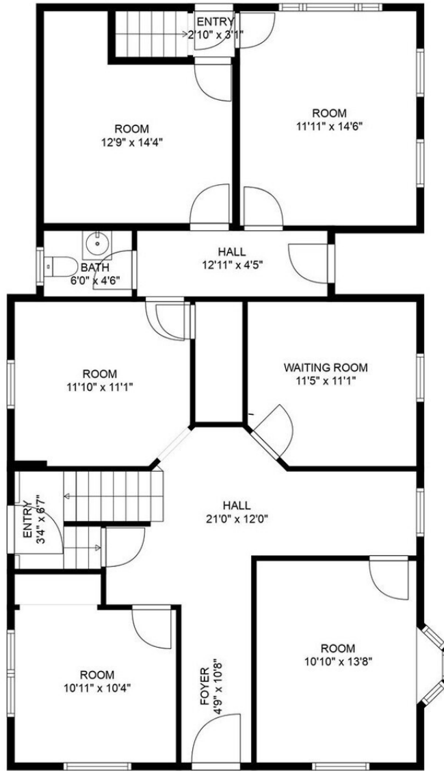
FLOOR 2
