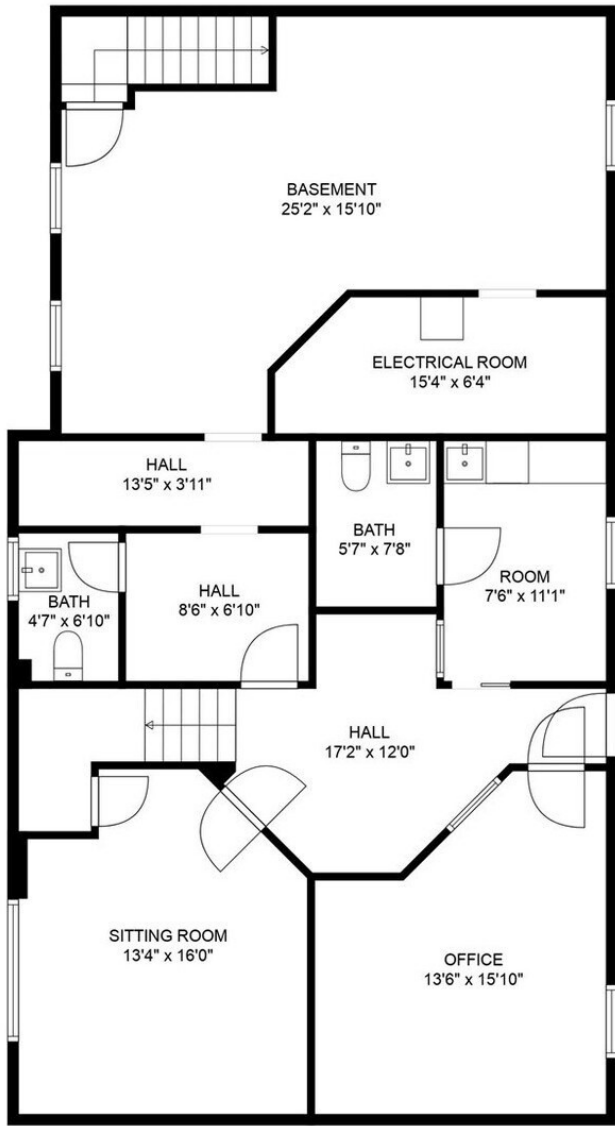
FLOOR 1
