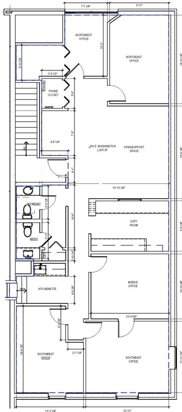
Second Floor Plan - 208 E. Washington
