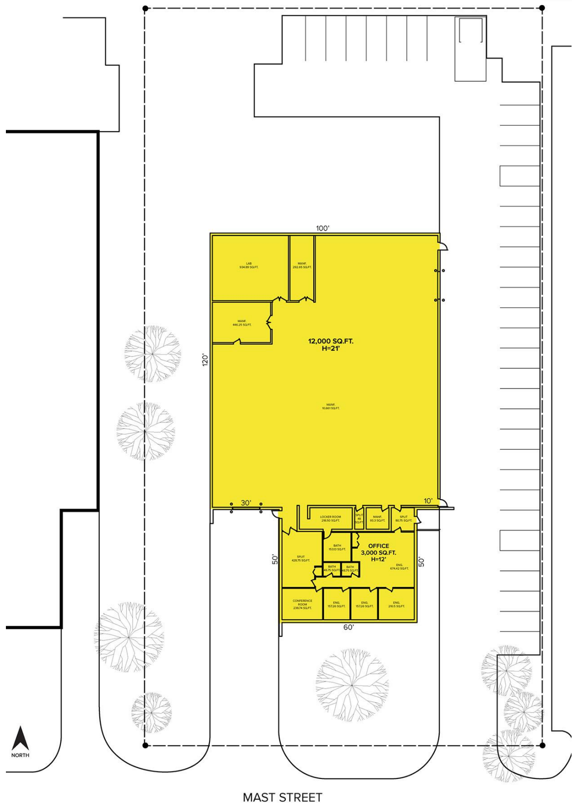
Site Plan
