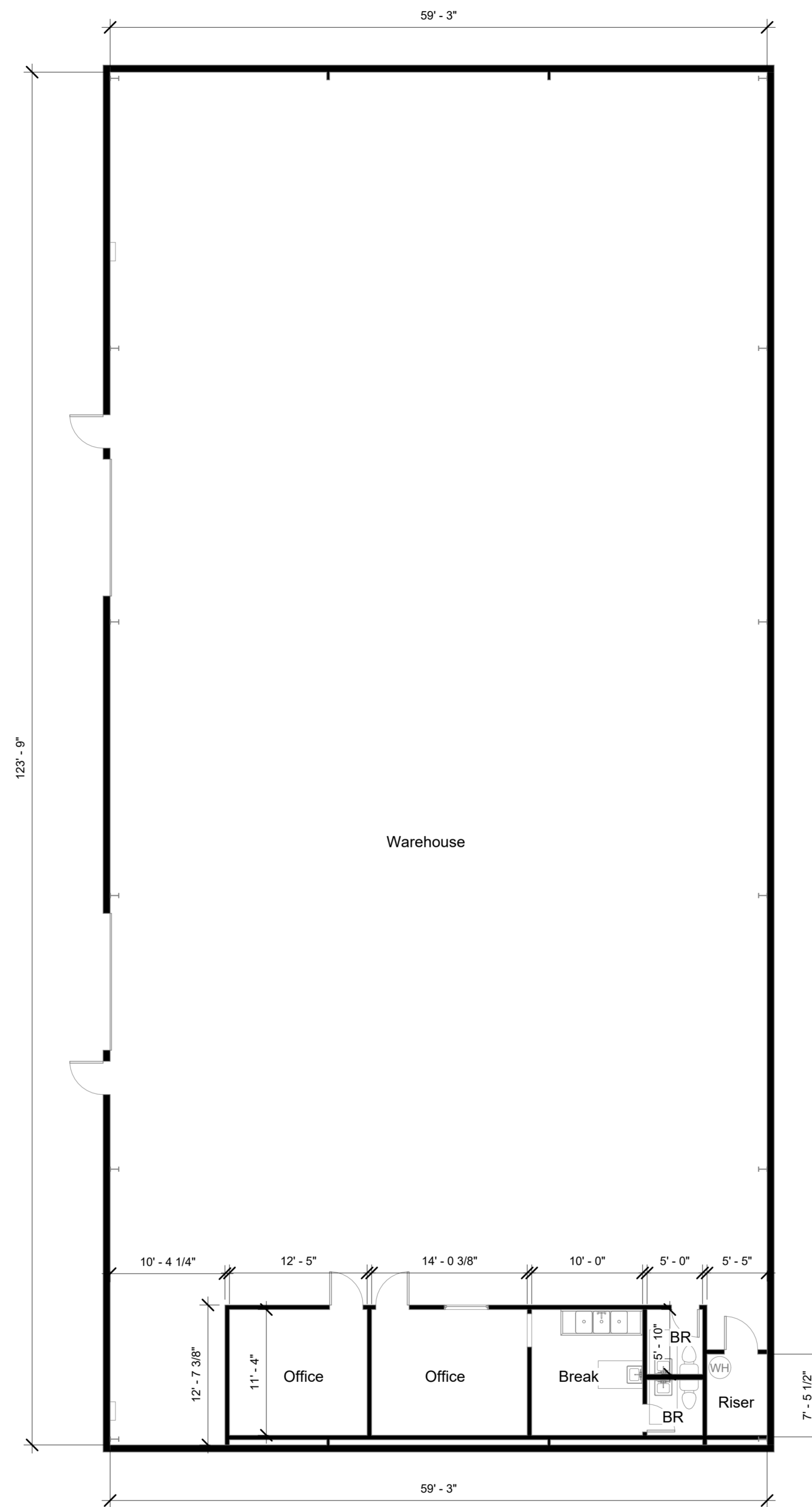
① Measured Plan - Dimensions 1/8" = 1'-0"
