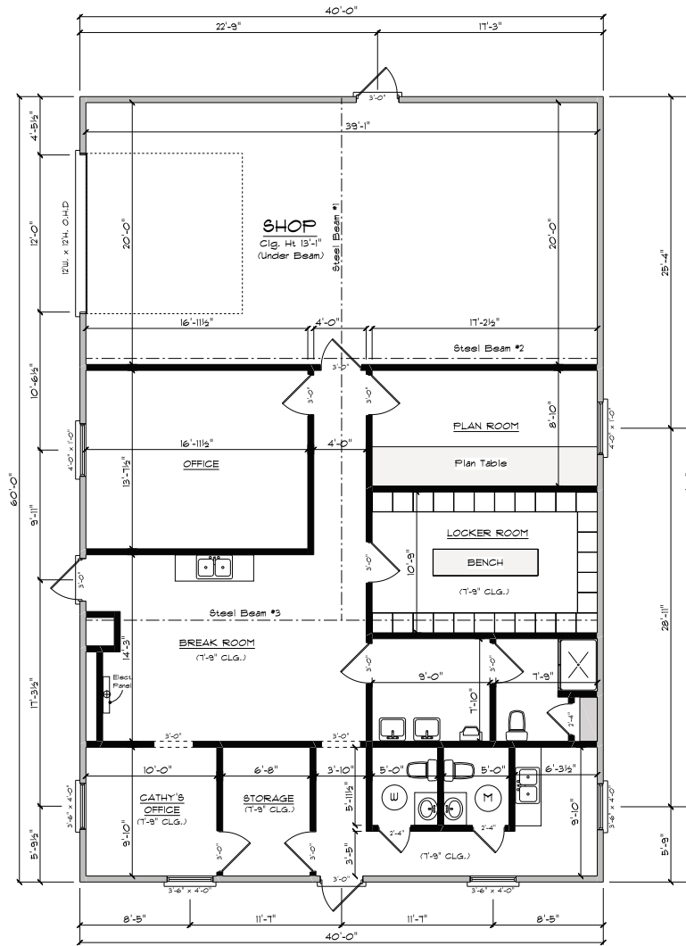
PROPOSED 1st FLOOR PLAN
