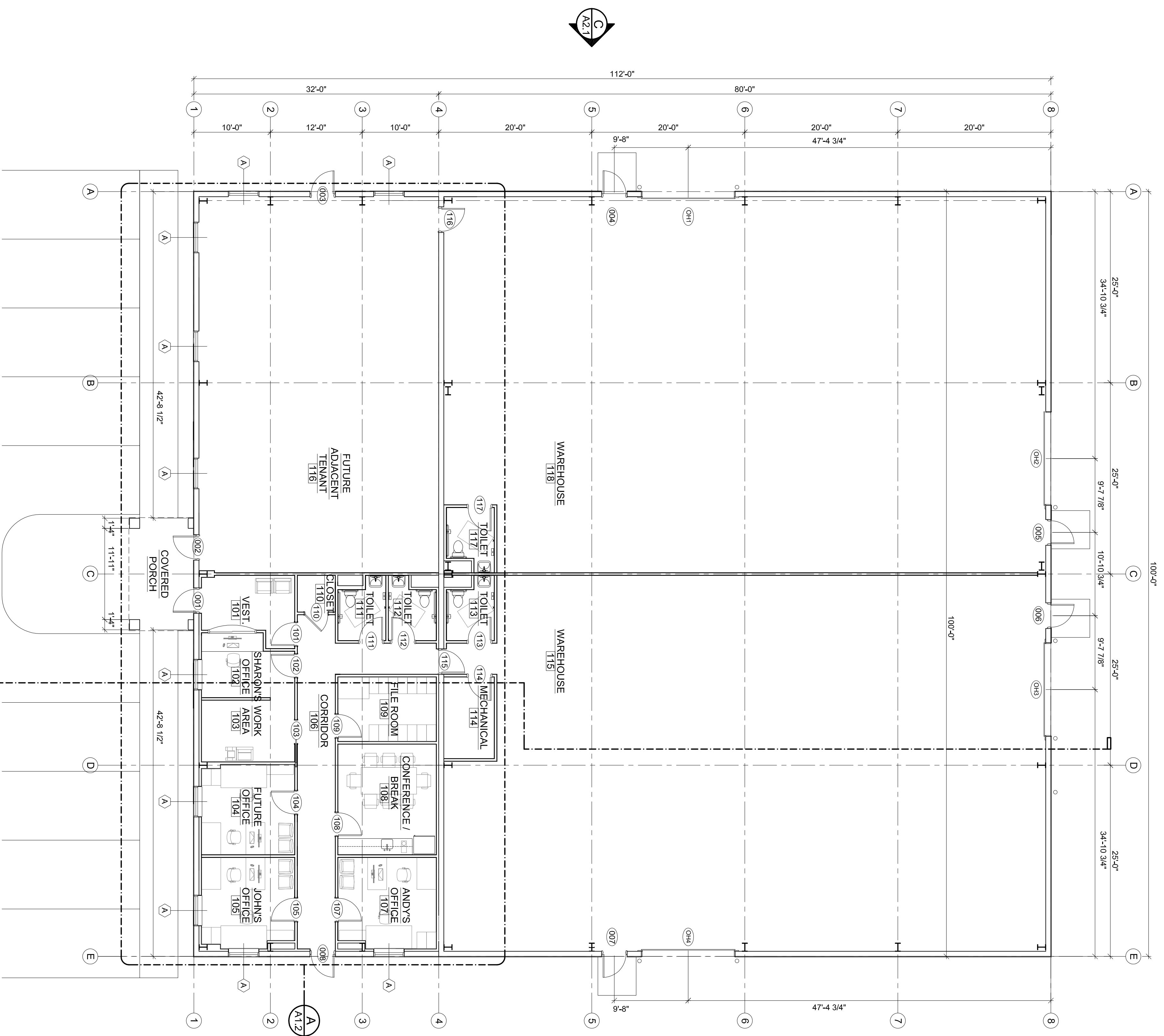
A OVERALL FLOOR PLAN A11 SCALE: 1/8" = 1'-0"
