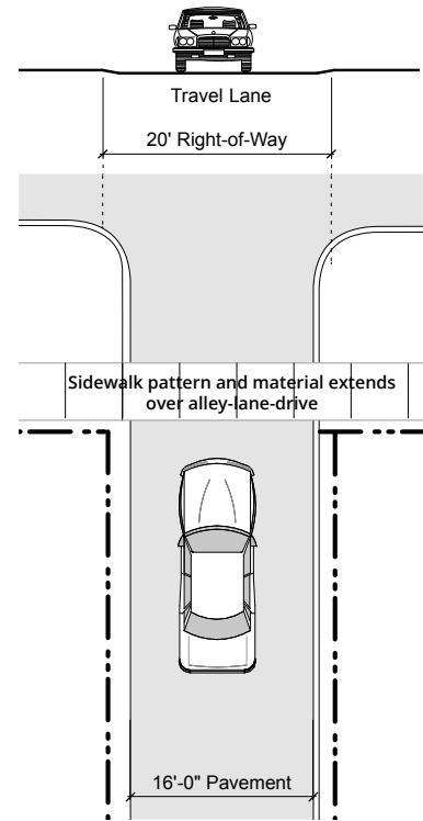
Figure 70.2.I-2. Typical Alley, Lane, or Service Drive
