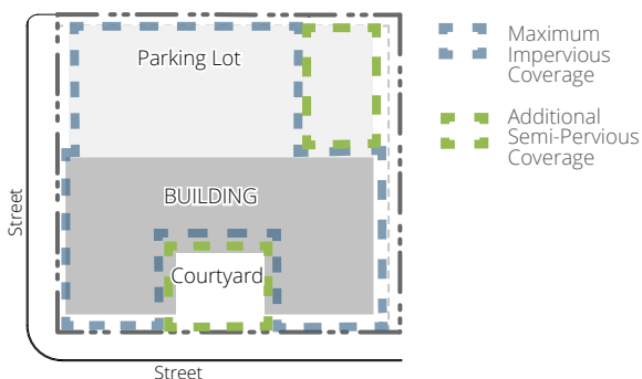
Figure 70.7.B-1. Site Impervious and Semi-Pervious Coverage
