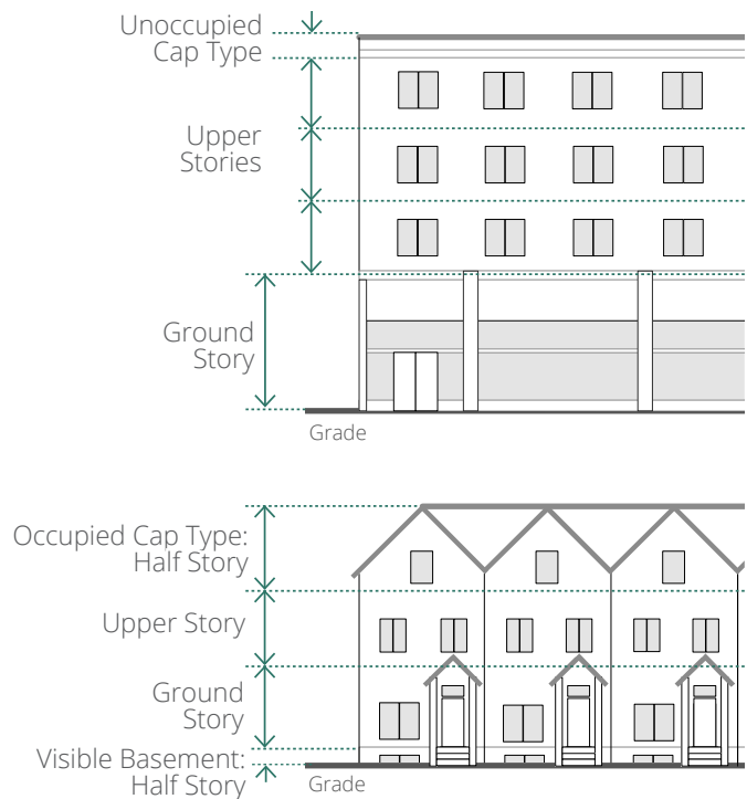
Figure 70.7.B-3. Measuring Stories with Floor-to-Floor Height
