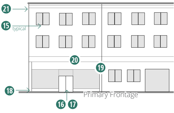
Figure 70.3.G-3. Workshop Building: Facade Design Requirements
