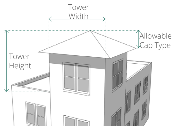
Figure 70.3.I-4. Example of a Tower
