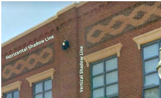
Figure 70.7.A-7. Examples of Shadow Lines
