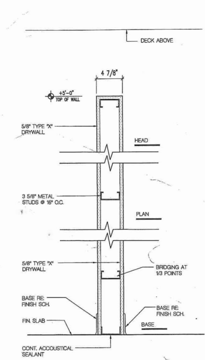
C 4" ACOUSTICAL DRYWALL - (NON-DEMISED) (STC 45) NO RATING
