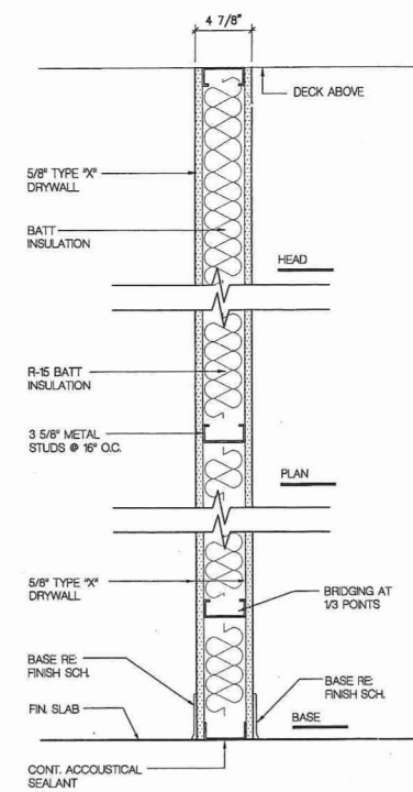
A 4" ACOUSTICAL DRYWALL - (DEMISED) (STC 45) NO RATING
