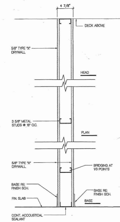
B 4" ACOUSTICAL DRYWALL - (DEMISED) NO RATING NO INSULATION
