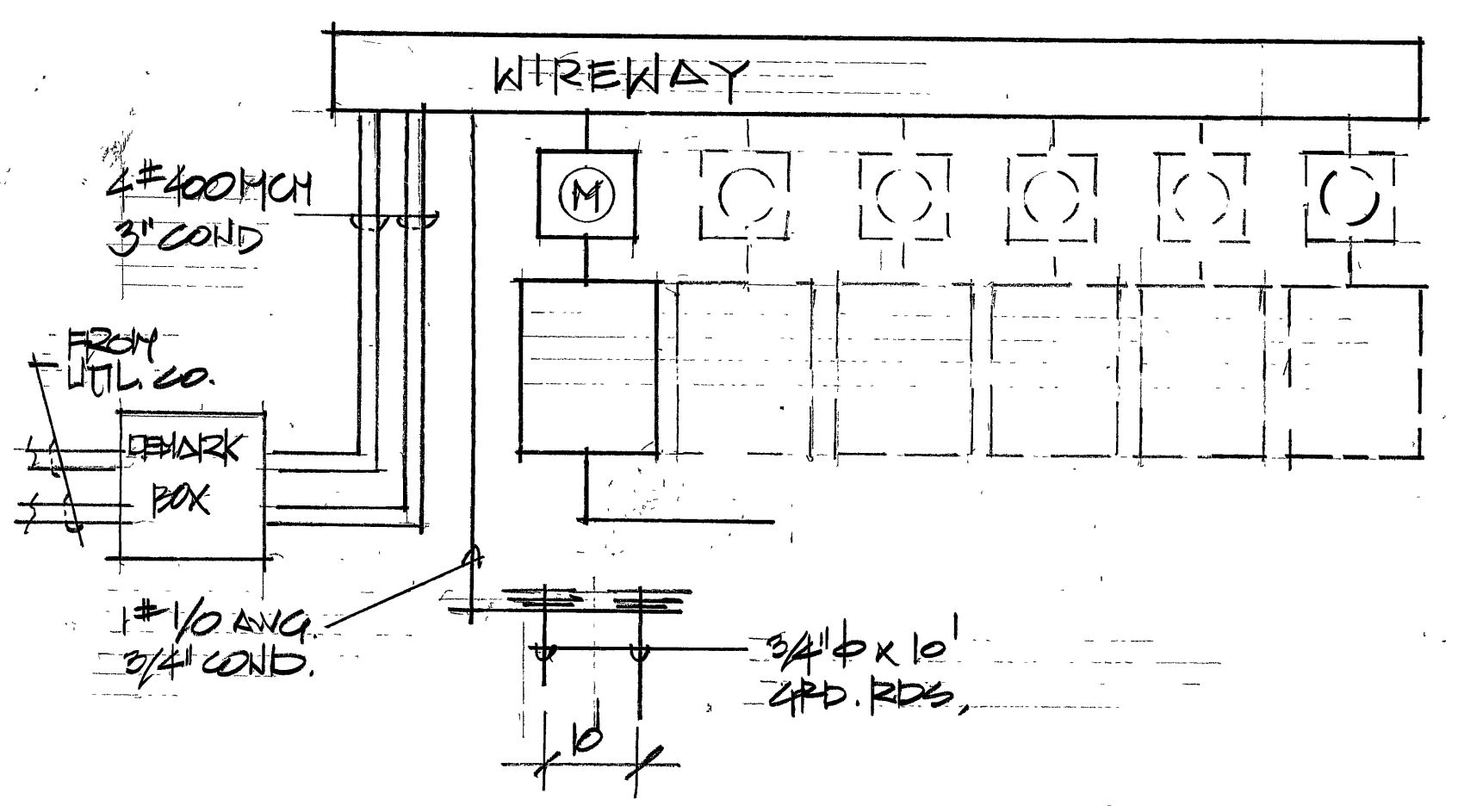
ELECTRICAL RISER DIAG
