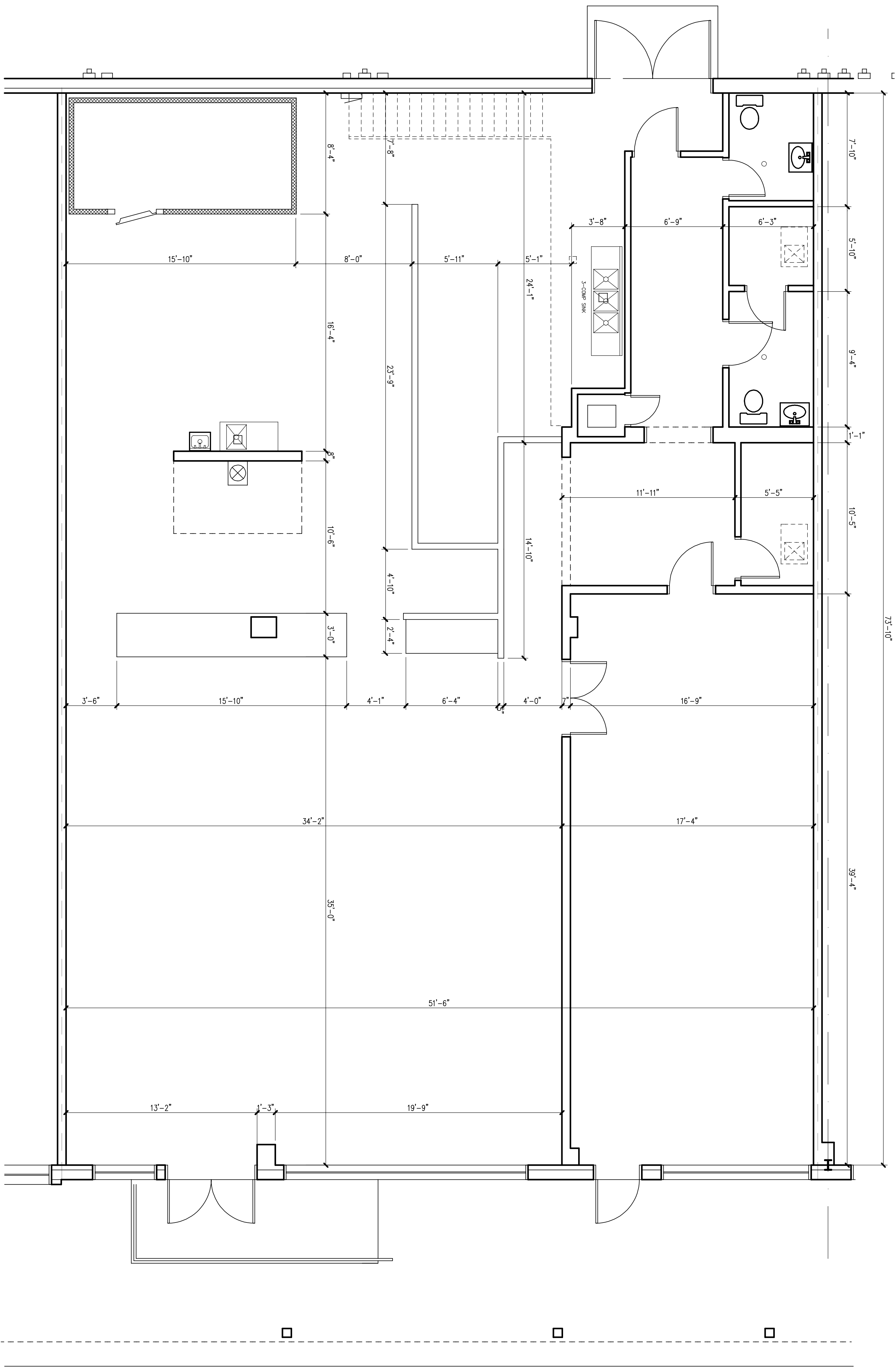
1 DIMENSIONED PLAN (FOX'S PIZZA) A2.3 1/4" = 1'-0"
