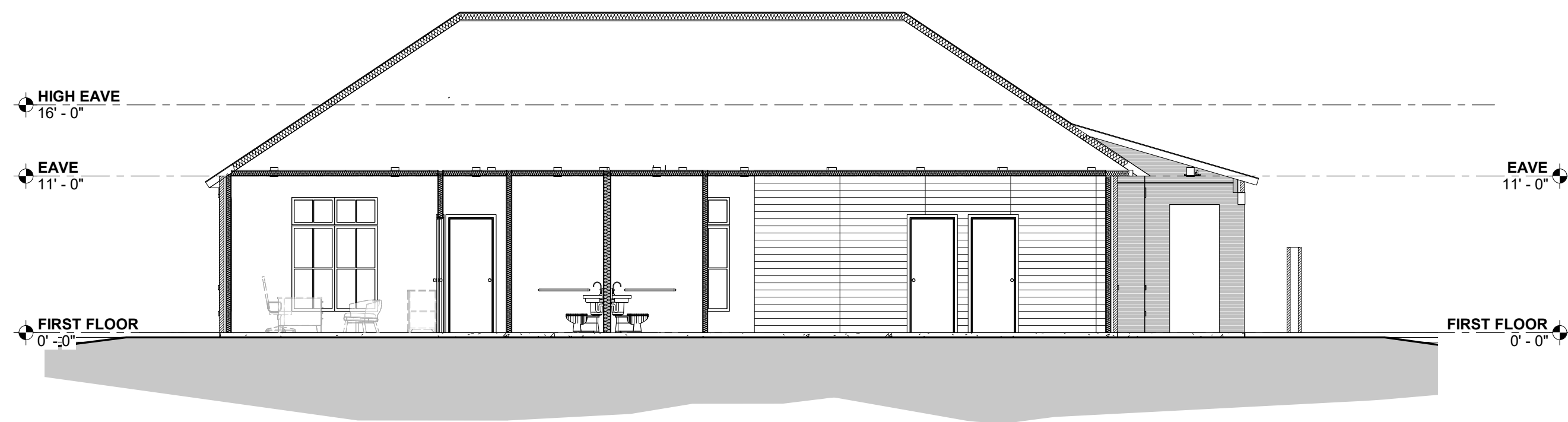
3 TRANSVERSE BUILDING SECTION SCALE: 0" = 1/8" = 1'-0"
