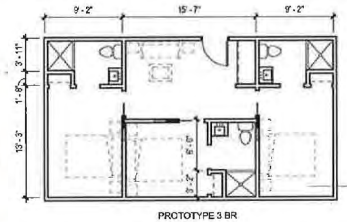
PROTOTYPE 3 BR
