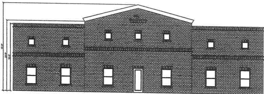
FRONT ELEVATION 3/16" SCALE
