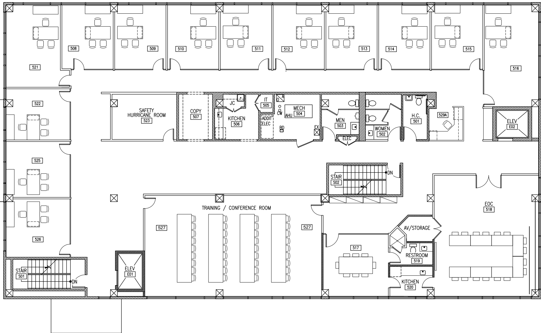
FIFTH FLOOR
