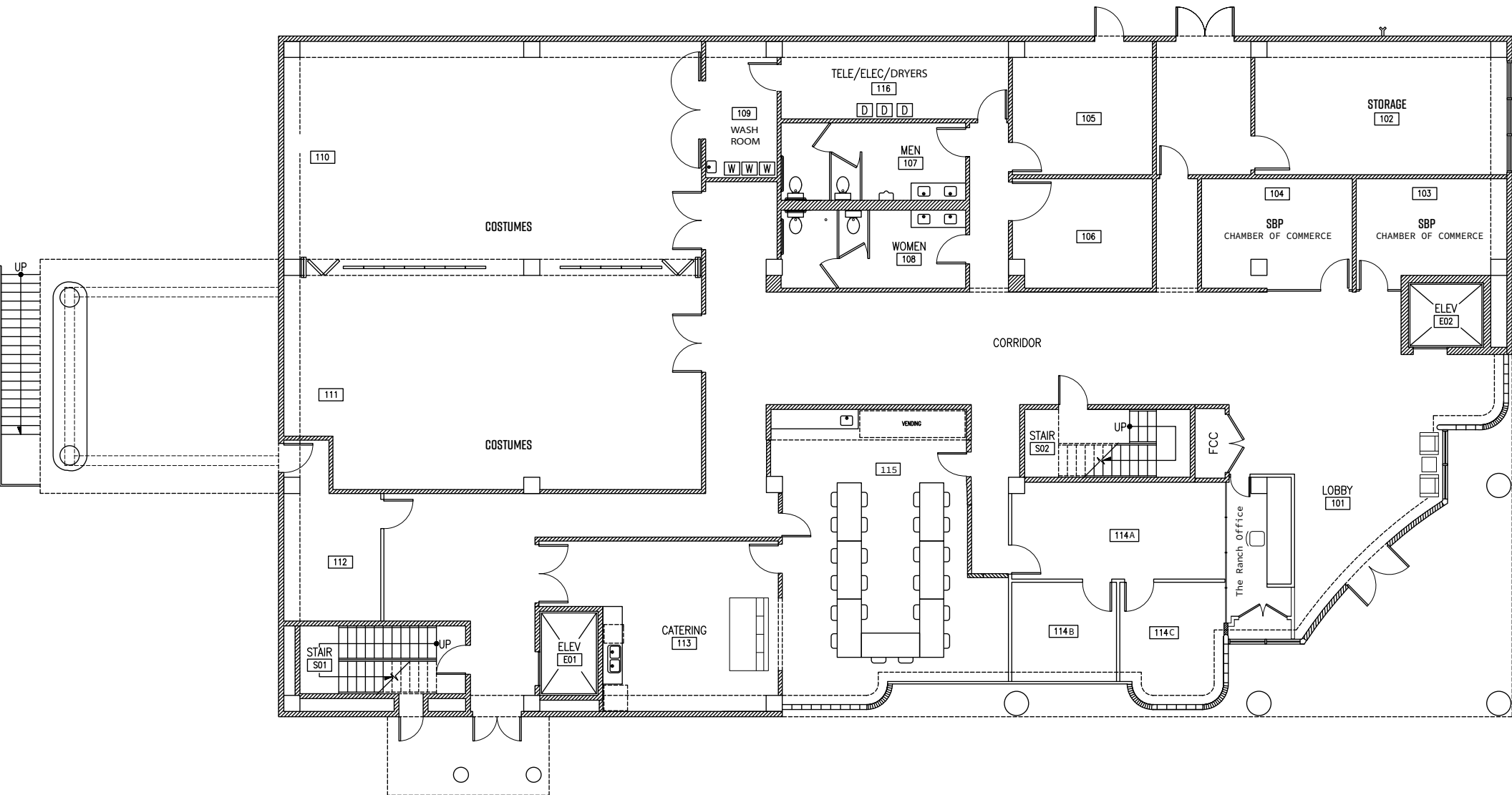
FIRST FLOOR
