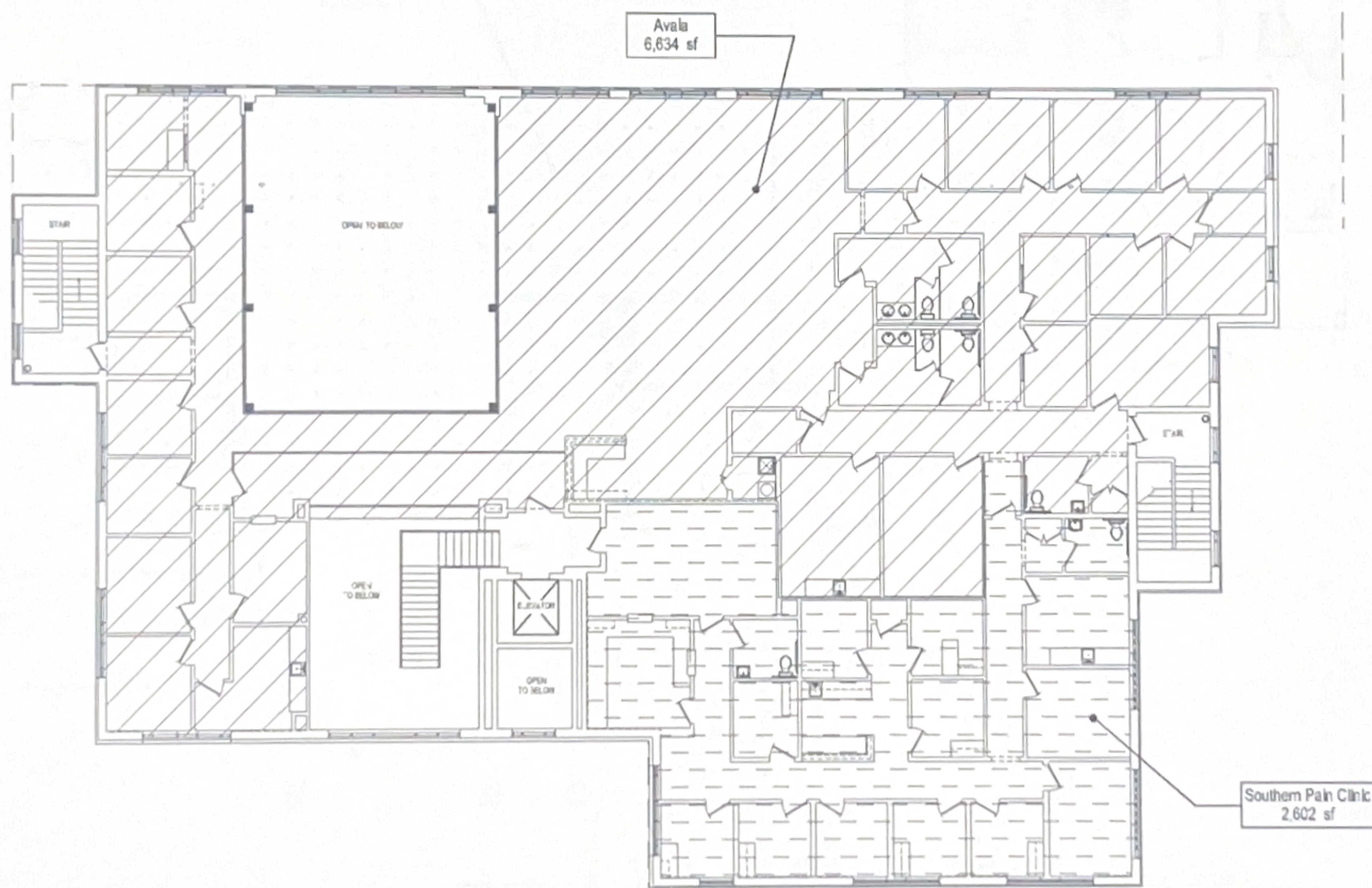
Existing Conditions Plan - 2nd Floor - 12,280 Gross Sf Scale: 1/8" = 1'-0"
