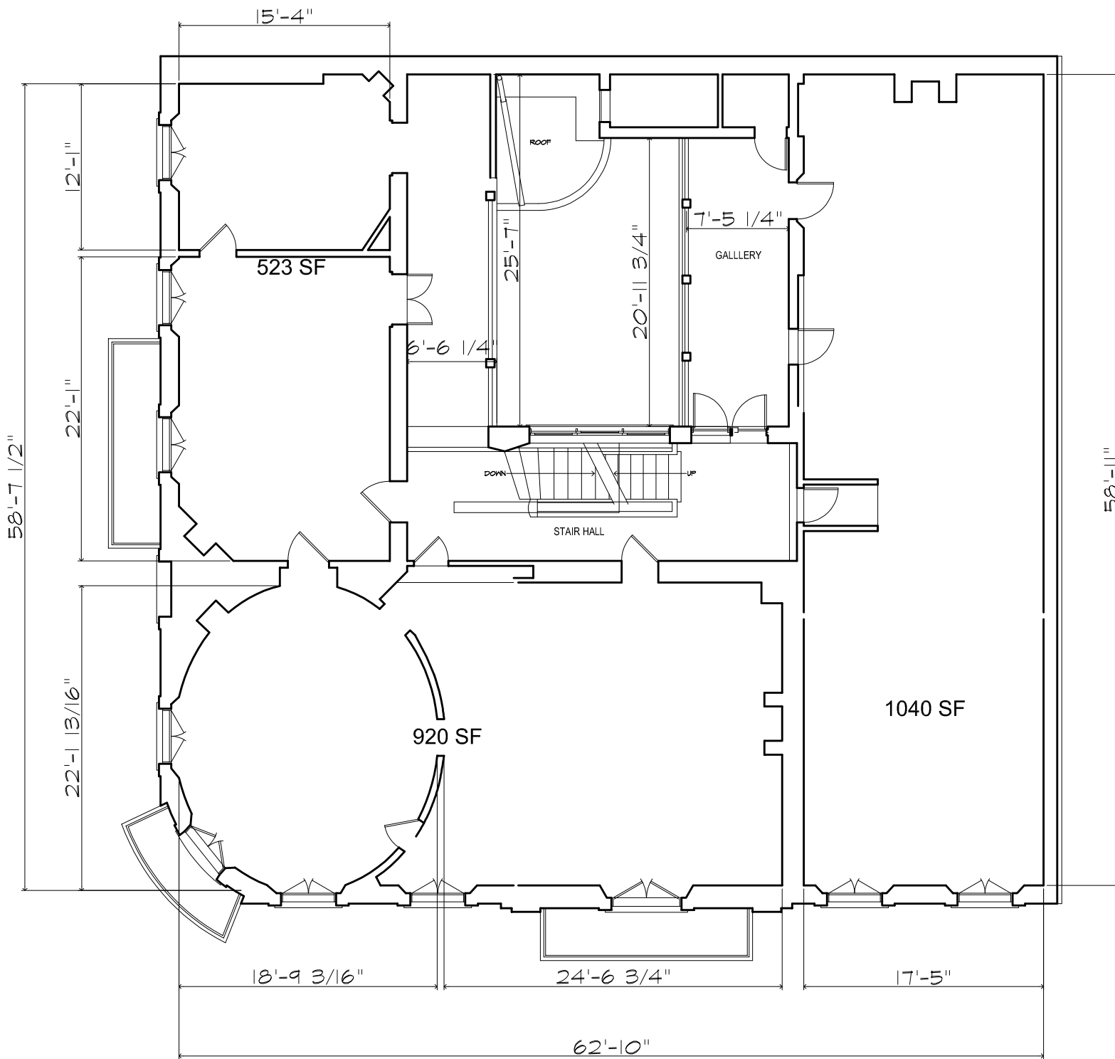
THIRD FLOOR
