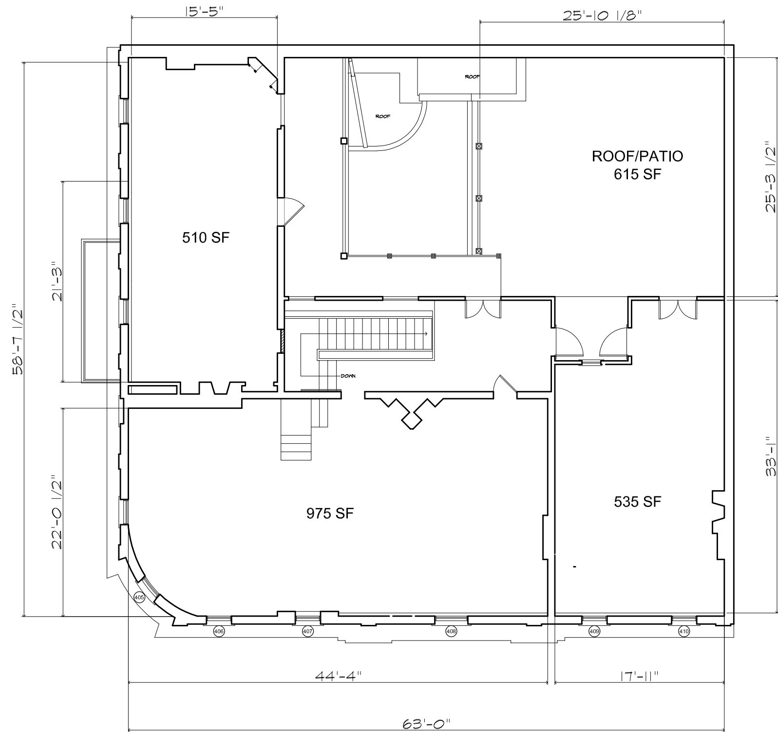
FOURTH FLOOR
