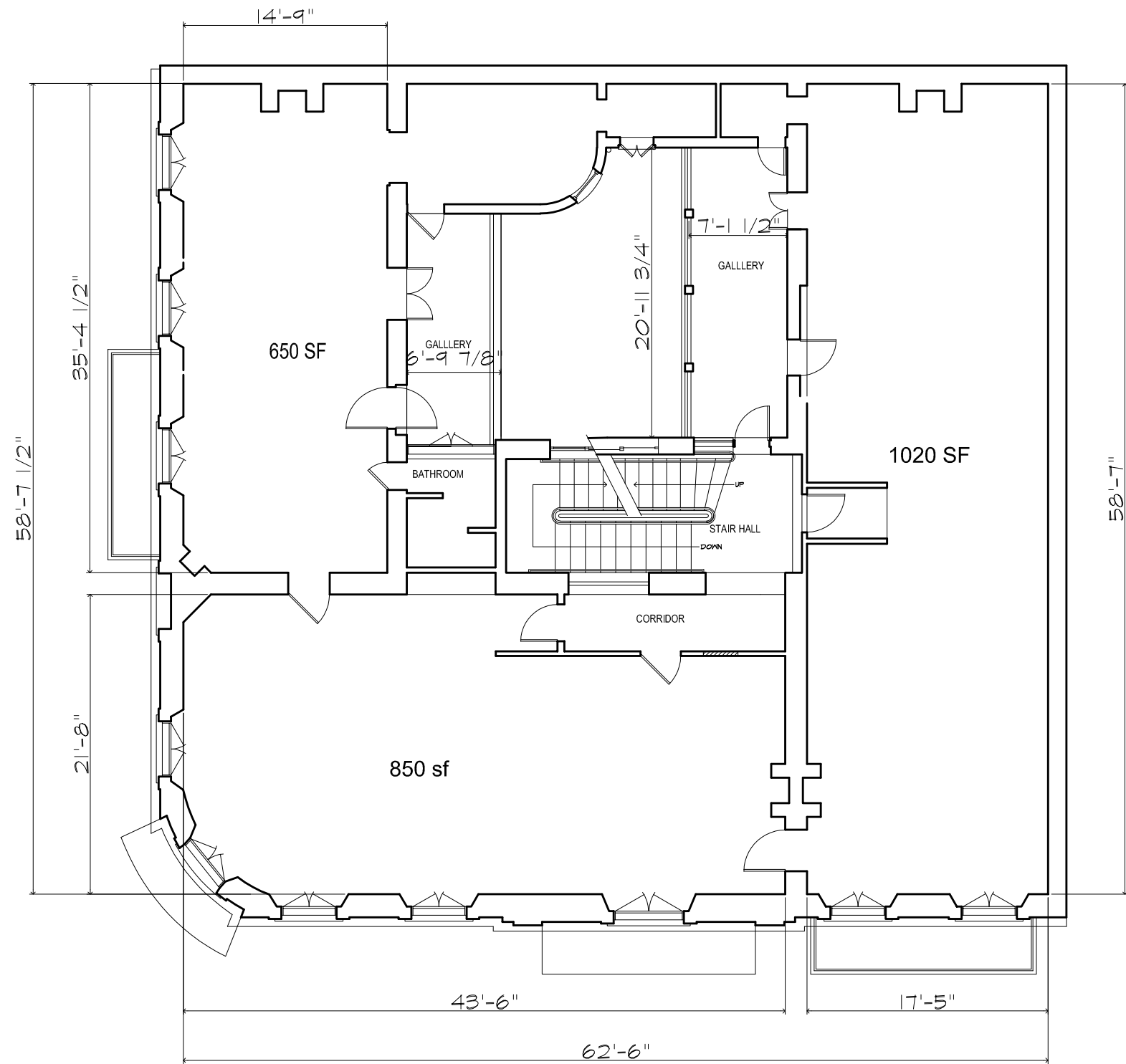
SECOND FLOOR
