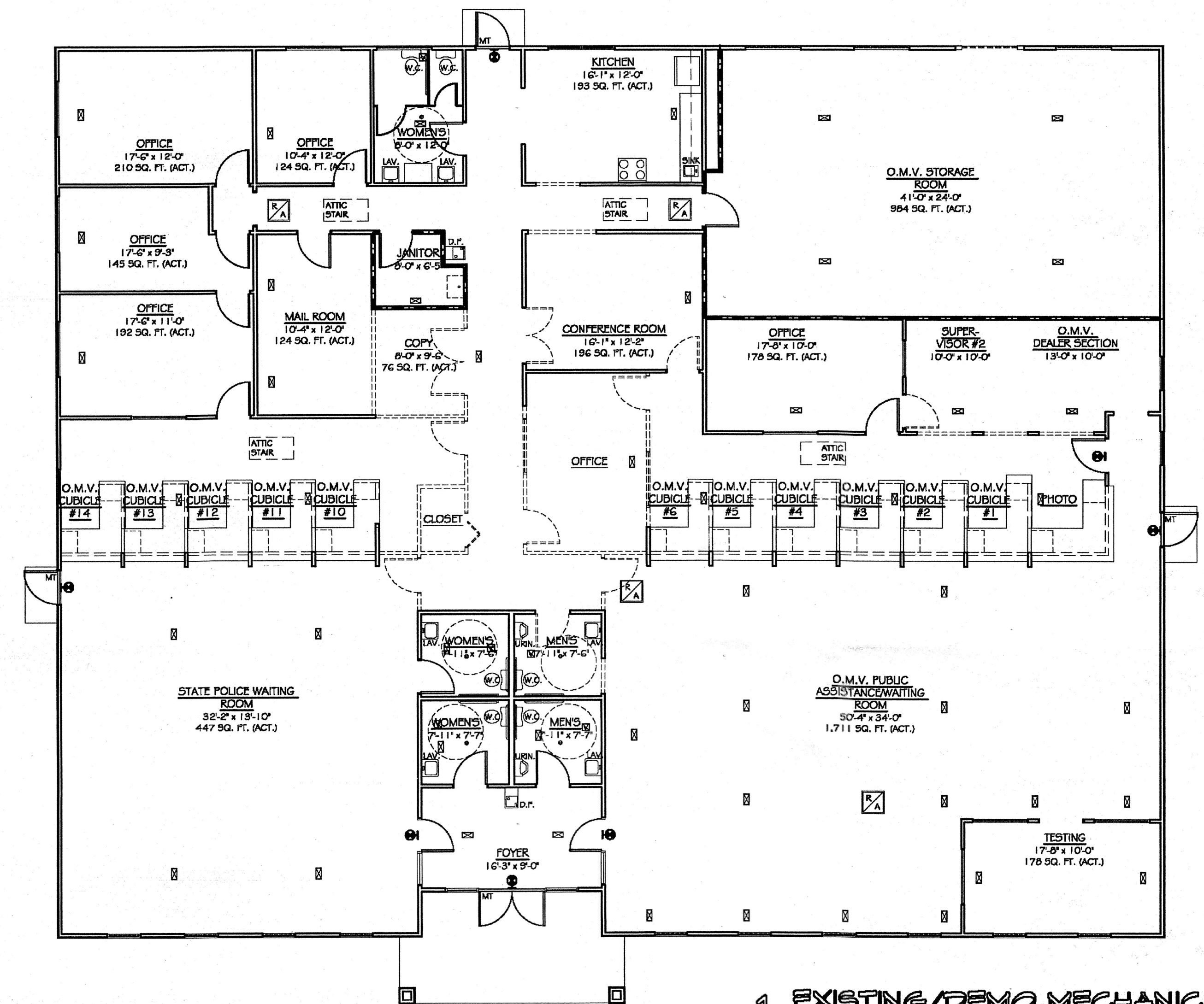
1. EXISTING/DEMO MECHANICAL PLAN SCALE: 1/8" = 1'-0"
