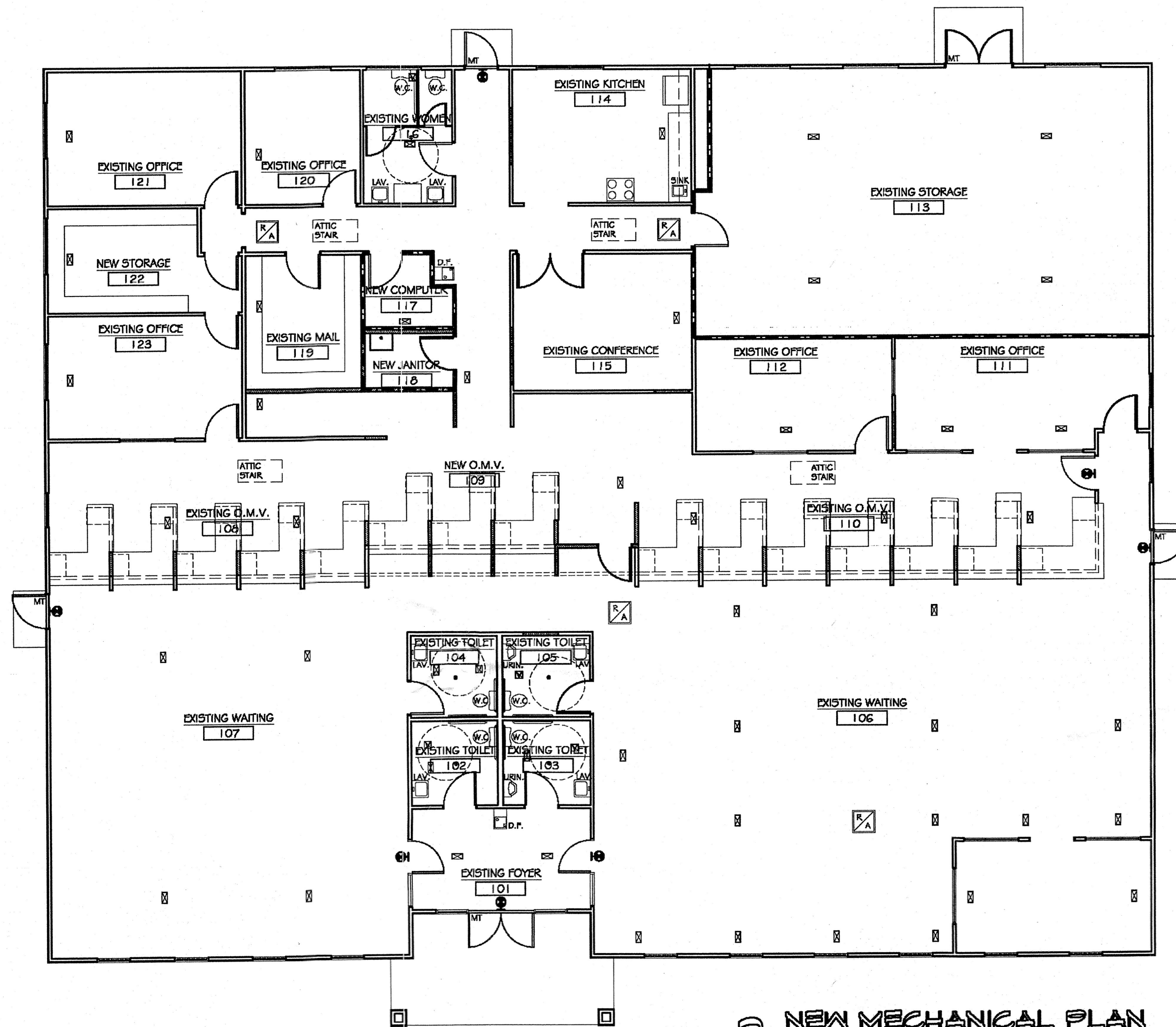
2. NEW MECHANICAL PLAN SCALE: 1/8" = 1'-0"
