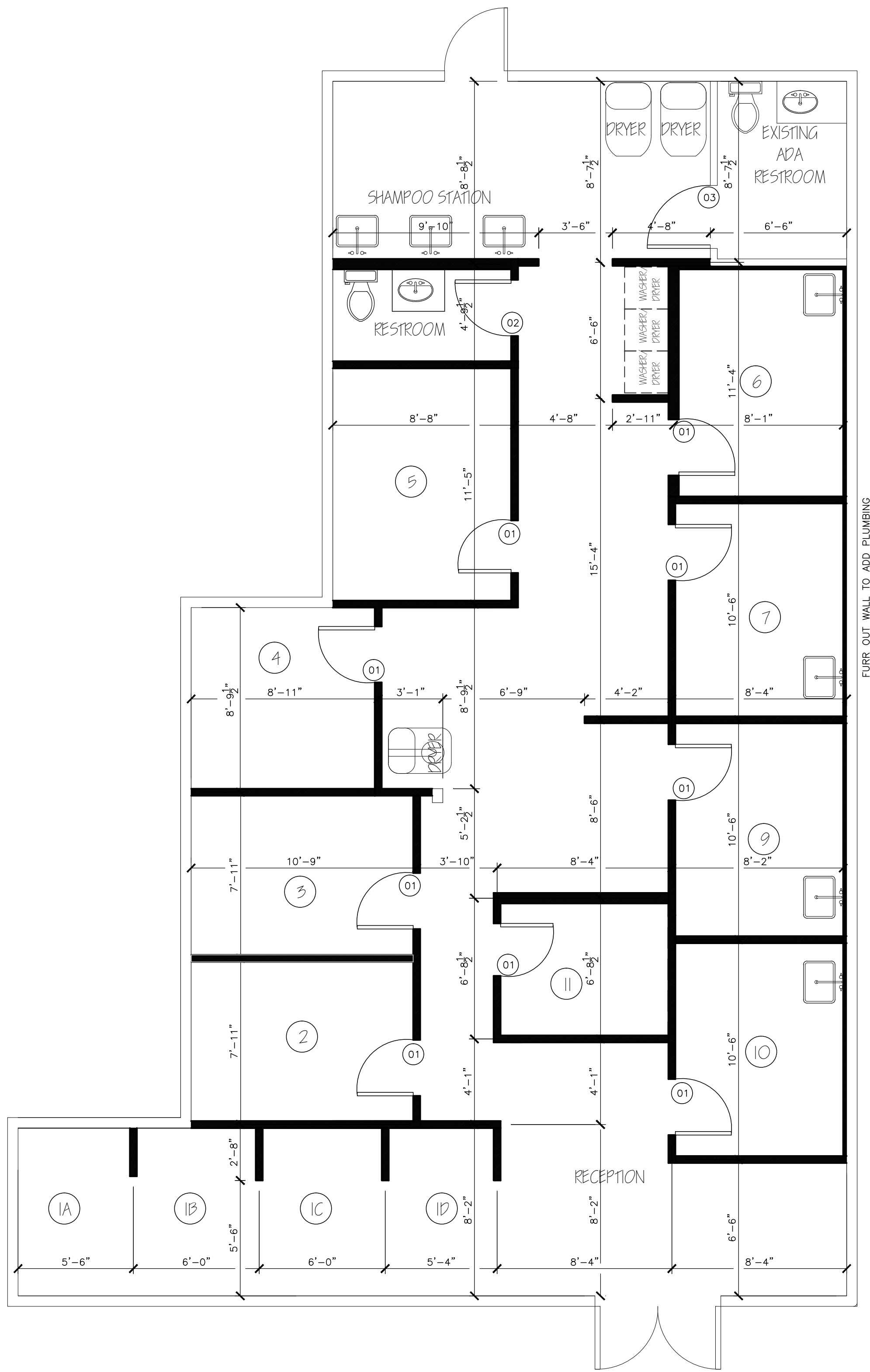
1 DIMENSIONED FLOOR PLAN 1/4"=1'-0"
