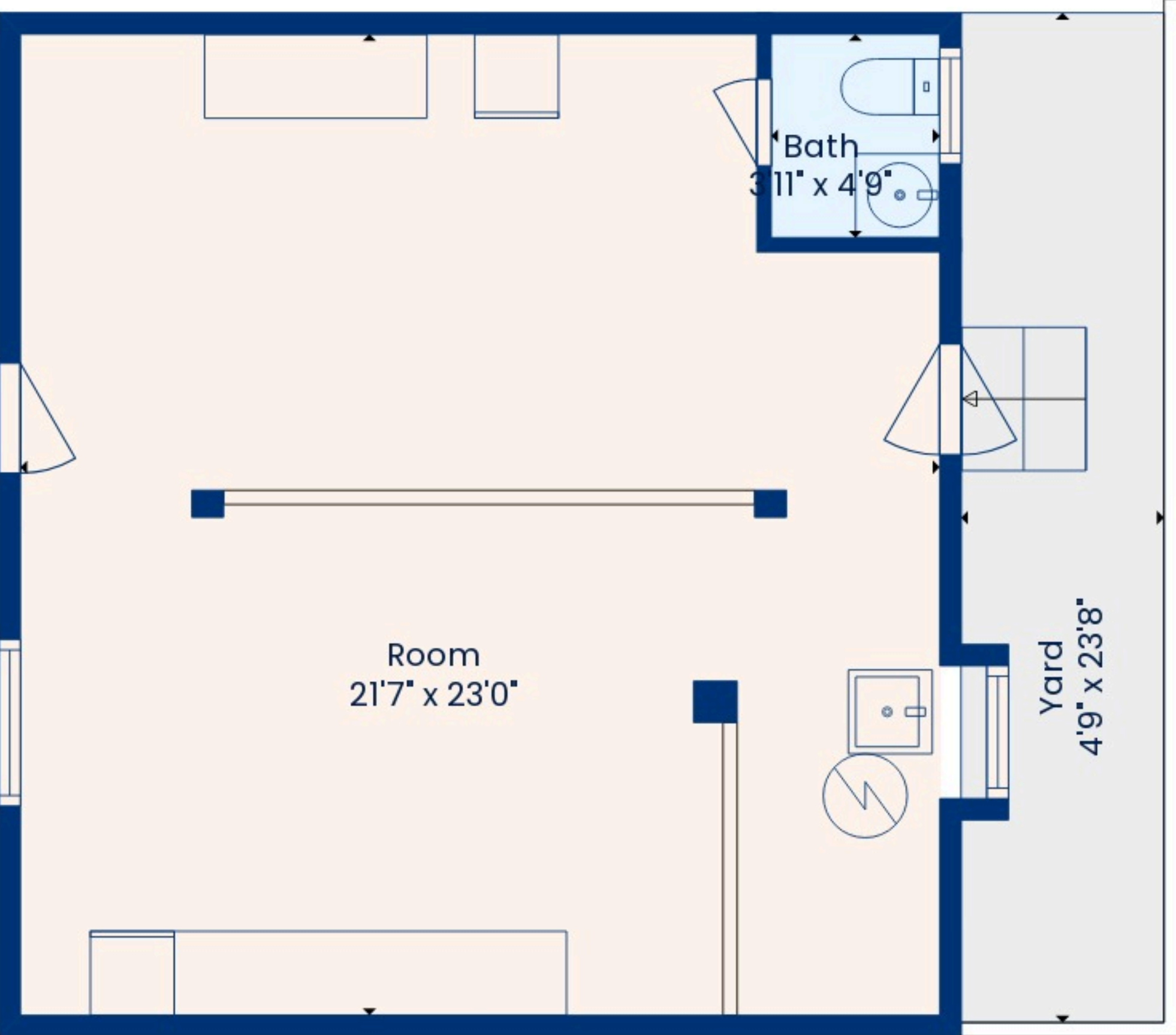
Floor 1
