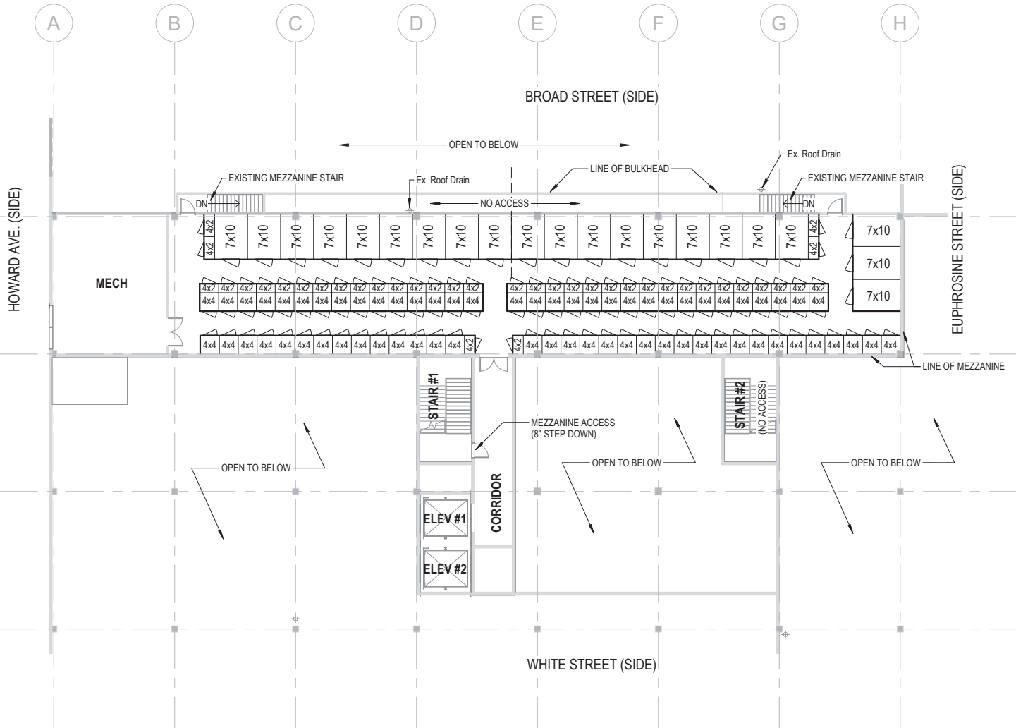
1 MEZZANINE PLAN 1/16" = 1'-0"
