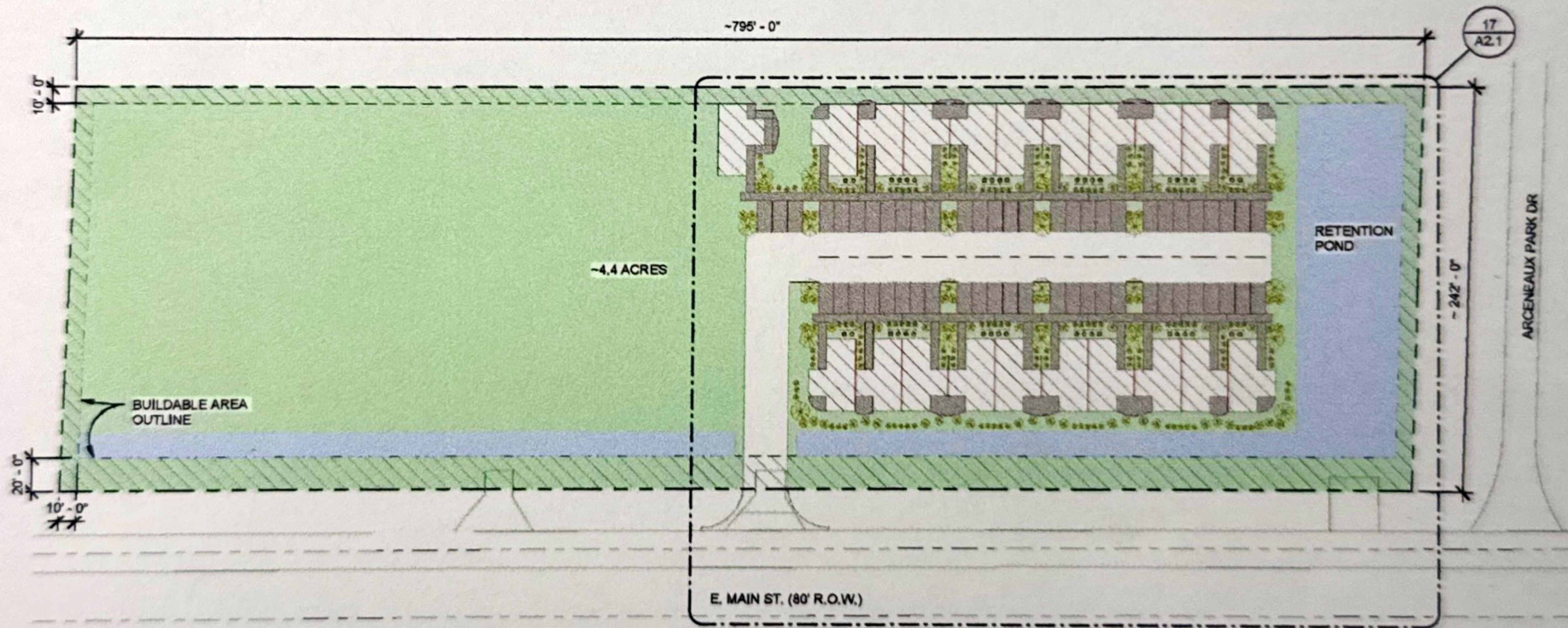
⑥ SITE PLAN - OVERALL PROPERTY 1" = 60'-0"
