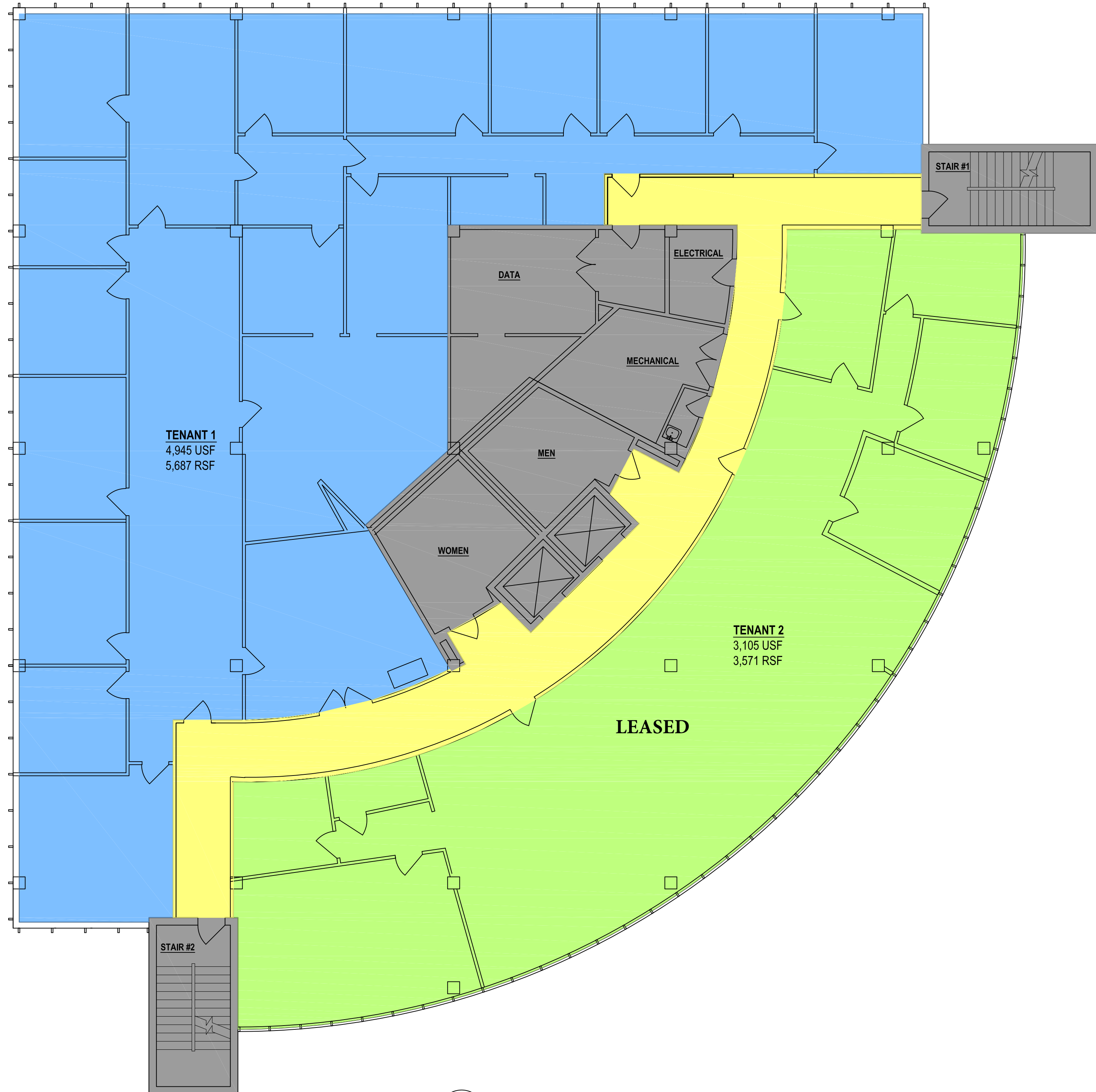
1 THIRD FLOOR PLAN-SCHEME A A1.00 1/8"= 1'-0"
