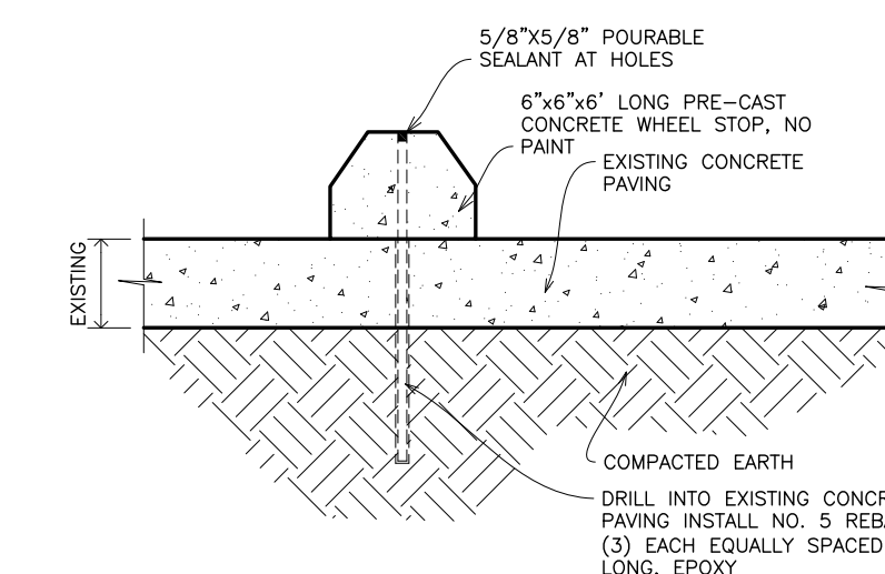
5 WHEEL STOP
