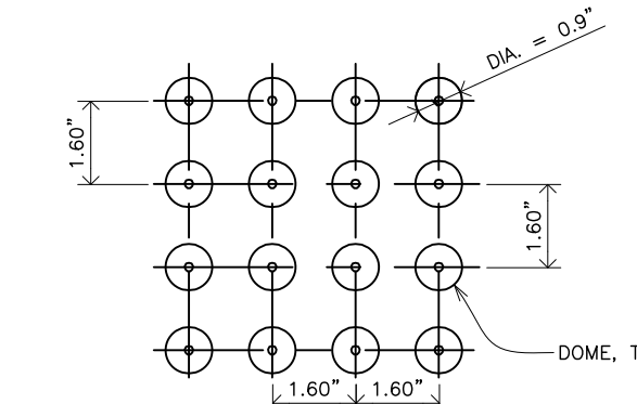
4 TRUNCATED DOMES SCALE: 3" = 1'-0"
